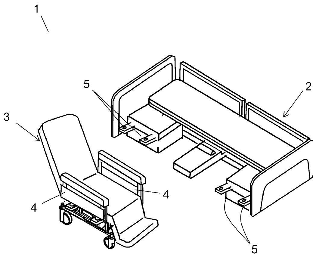
FIG. 8 PRIOR ART
