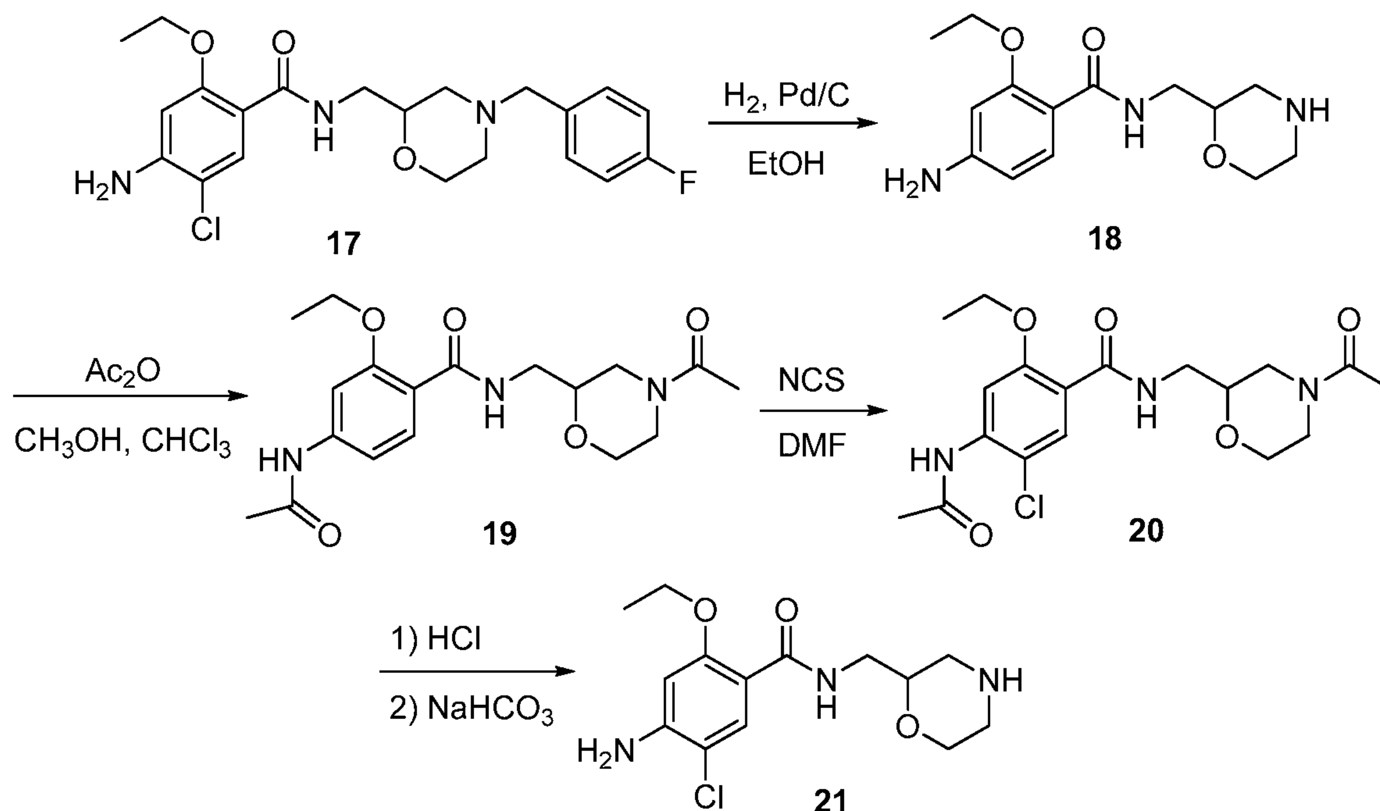
Scheme VI: Synthesis of Intermediate 21.
