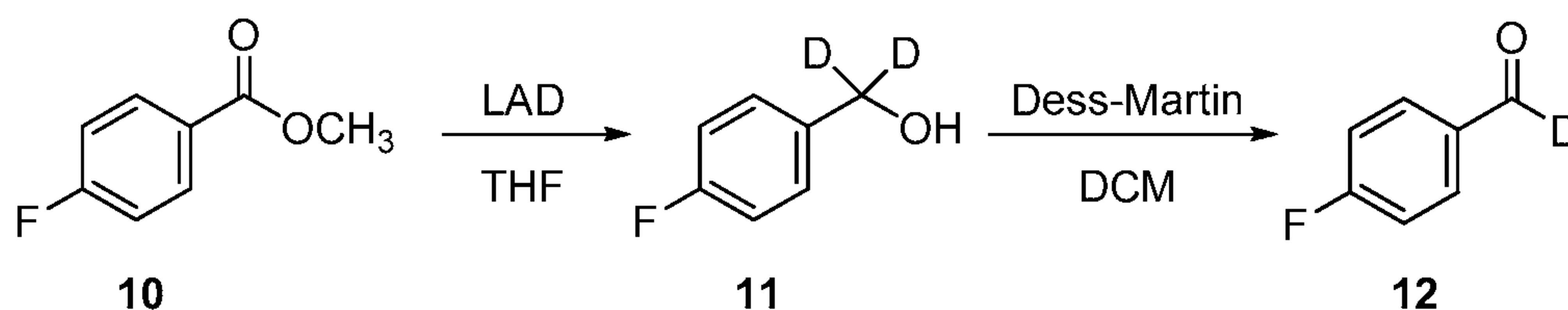
Scheme IV: Synthesis of Intermediate 12.
