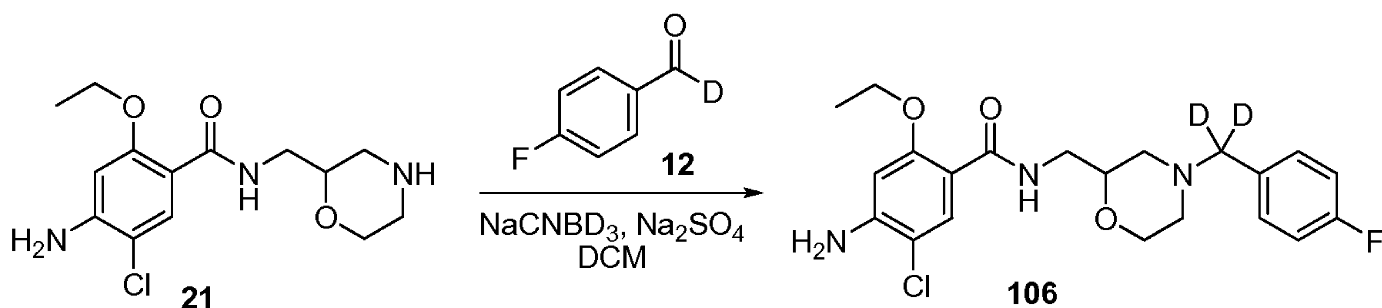
Scheme VII: Synthesis of Compound 106.
