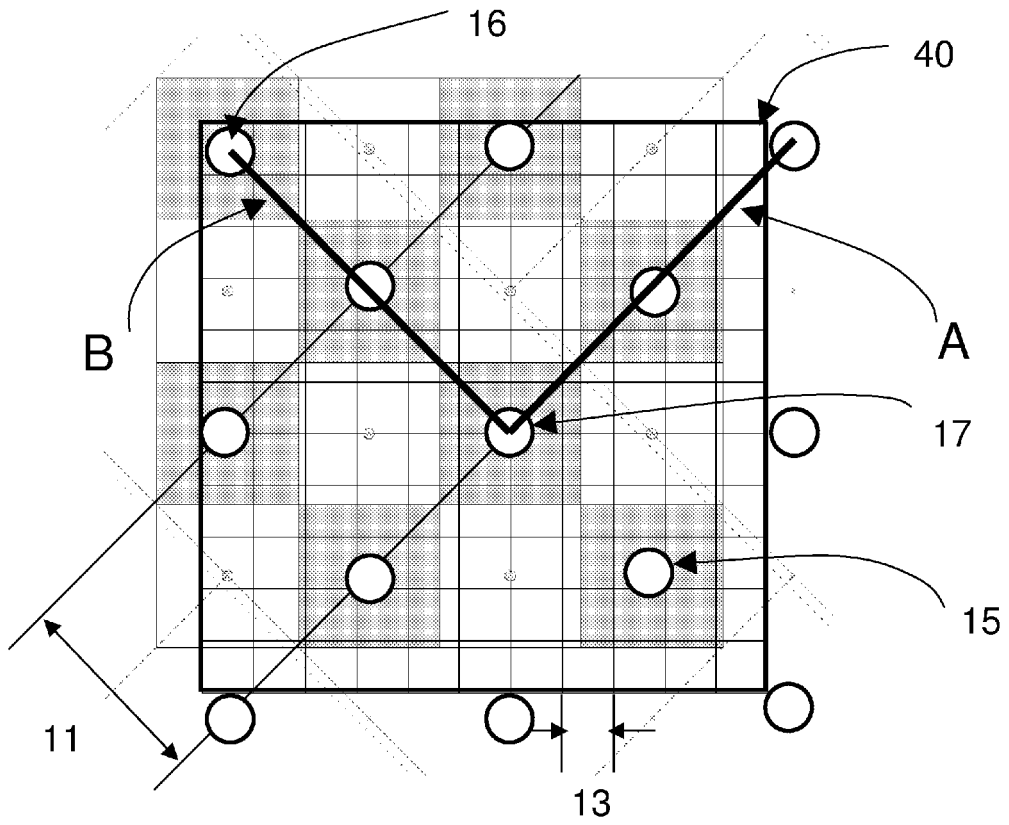
Fig 3 prior art
