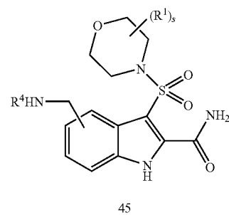
SCHEME 17
