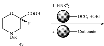
SCHEME 18
