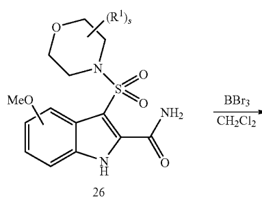
SCHEME 6
