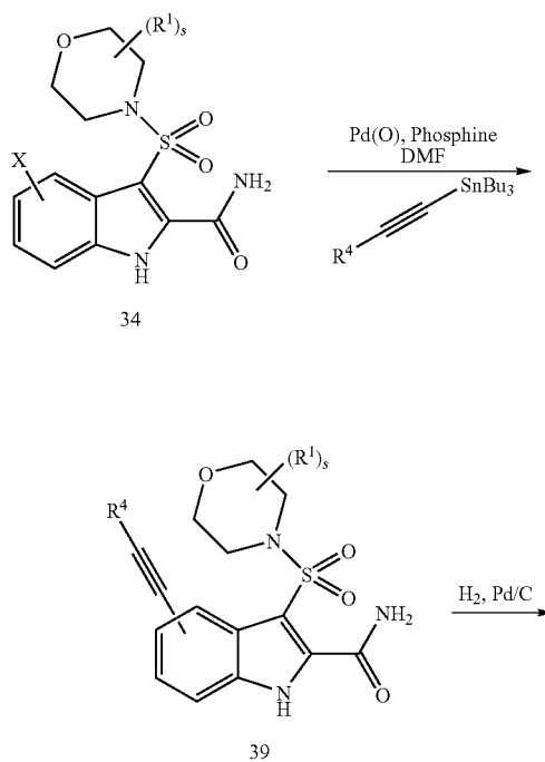
SCHEME 14
