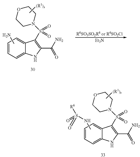
SCHEME 9
