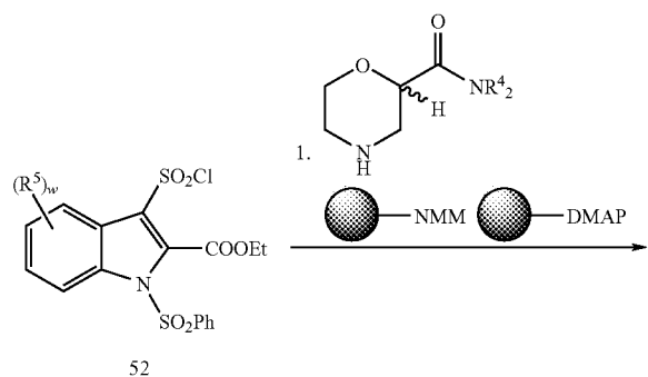
SCHEME 19
