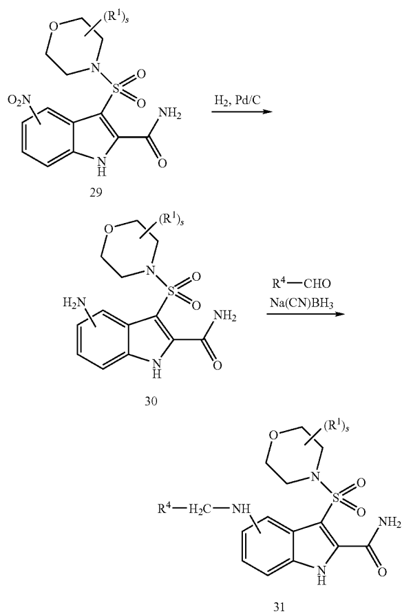
SCHEME 7
