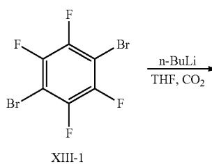
Scheme 13
