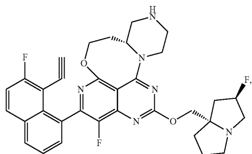
Trans mixture
