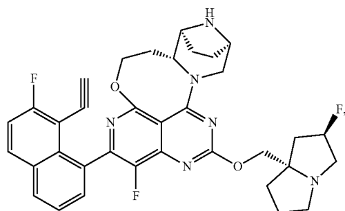
Cis mixture
