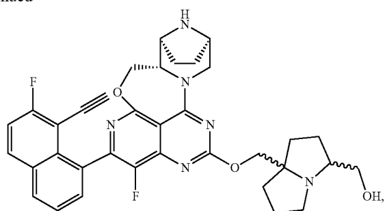
Cis mixture
