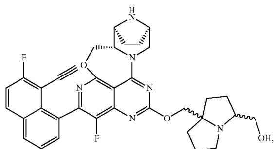
Trans mixture
