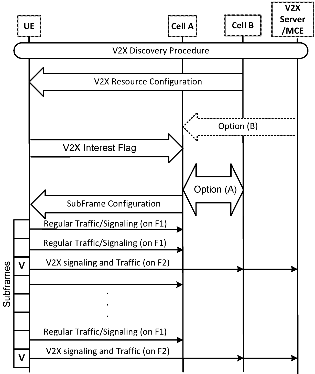
Time/Subframe Multiplexing Between F1 and F2
