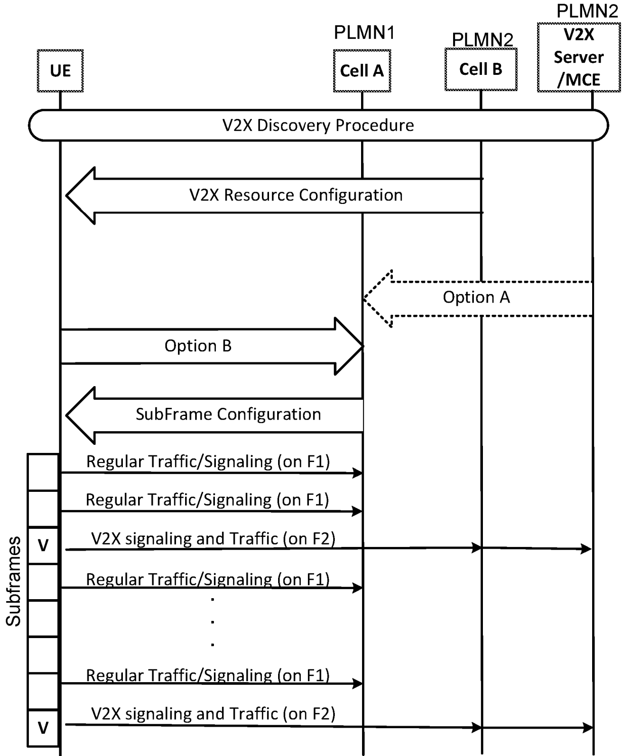
Time/Subframe Multiplexing Between F1 and F2
