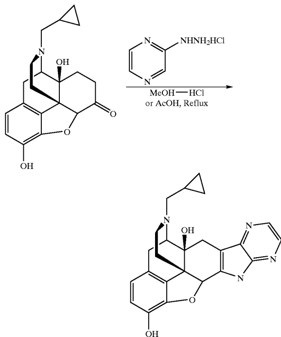
Scheme 6. Possible Synthetic Pathway of OP-44
