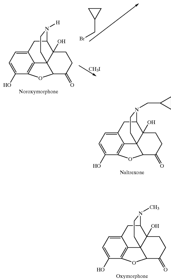
Scheme 1. General Synthetic Pathway of Oxymorphone and Naltrexone
