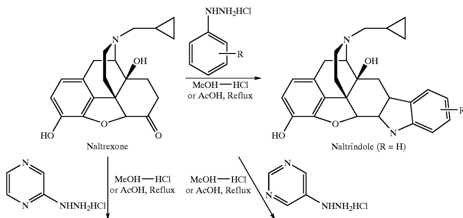
Scheme 5. Summarized Synthetic Pathway of OP-44 derivatives
