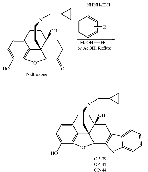
Scheme 2. General Synthetic Scheme of Naltrindole Derivatives
