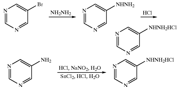
Scheme 7. General Synthetic Pathway of Hydrazine-HCl Salts
