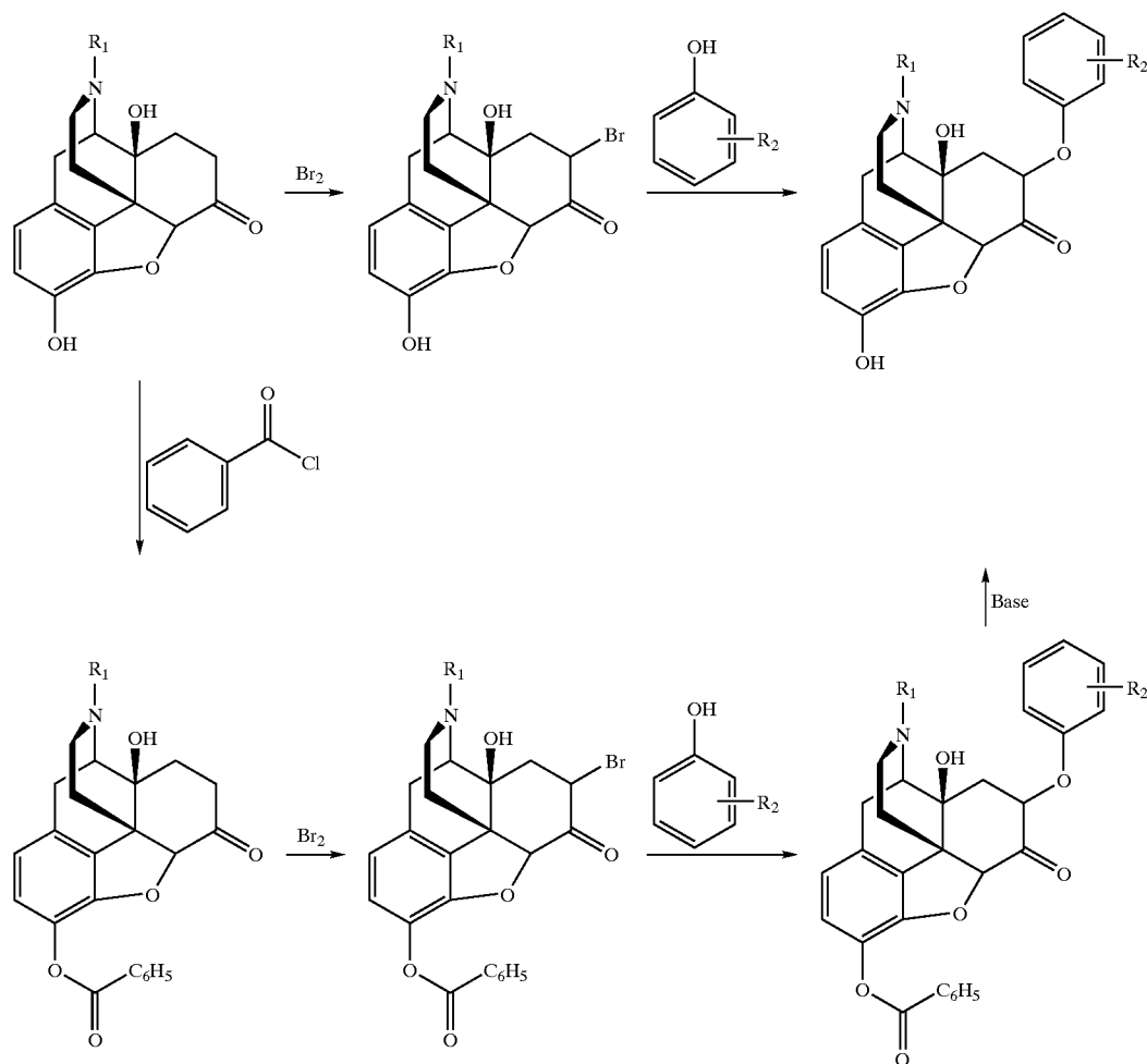
Scheme 4. Possible Synthetic Pathway of OP-26 Derivatives
