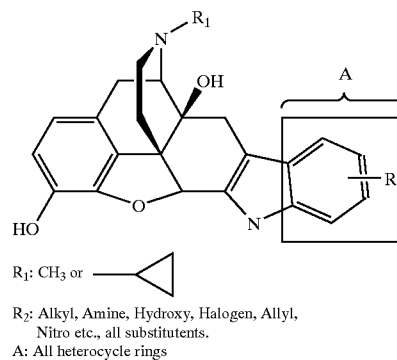
Scheme 3. Possible Modification of OP-44 Derivatives Based on General Synthetic Pathway
