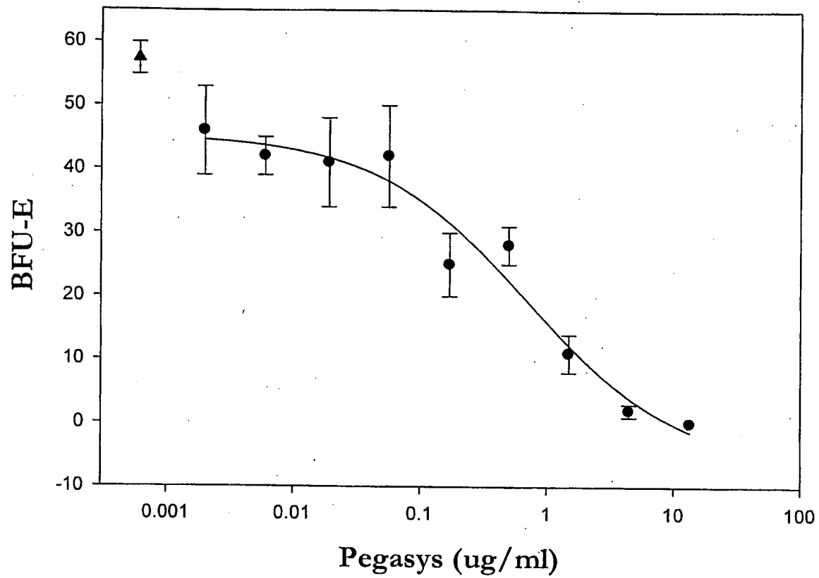
Figure 12 Pegasys, BFU-E
