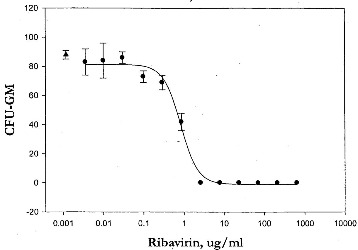
Figure 16 Ribavirin, CFU-GM
