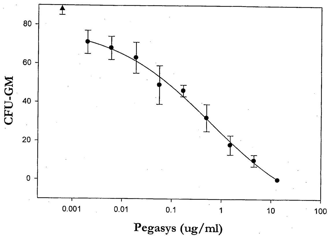
Figure 13 Pegasys, CFU-GM
