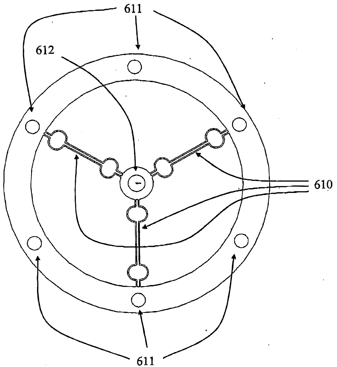
12 FIG. 12 Planar flexures schemes for assembled flexure scheme.
