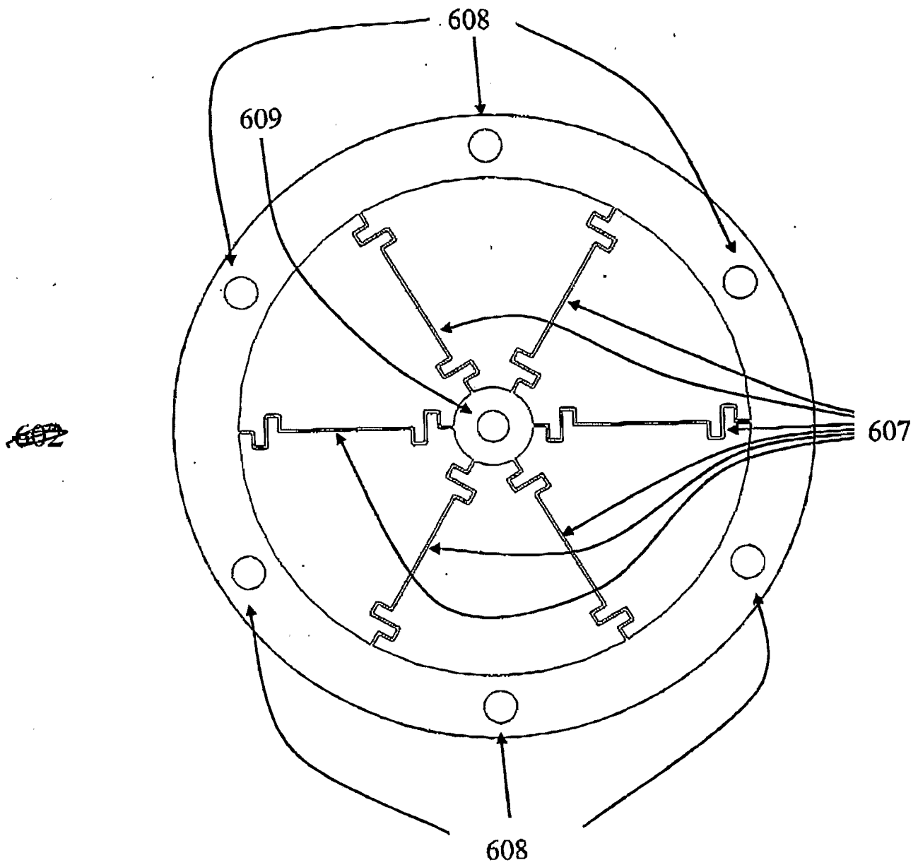
FIG. 11 Planar flexures schemes for assembled flexure scheme.
