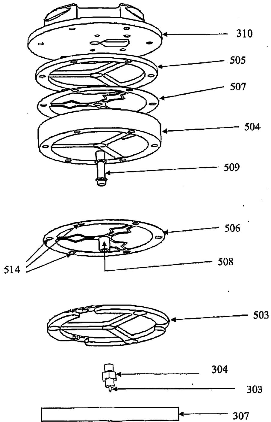
FIG. 8 Nanoindenter schema 2 before assembly
