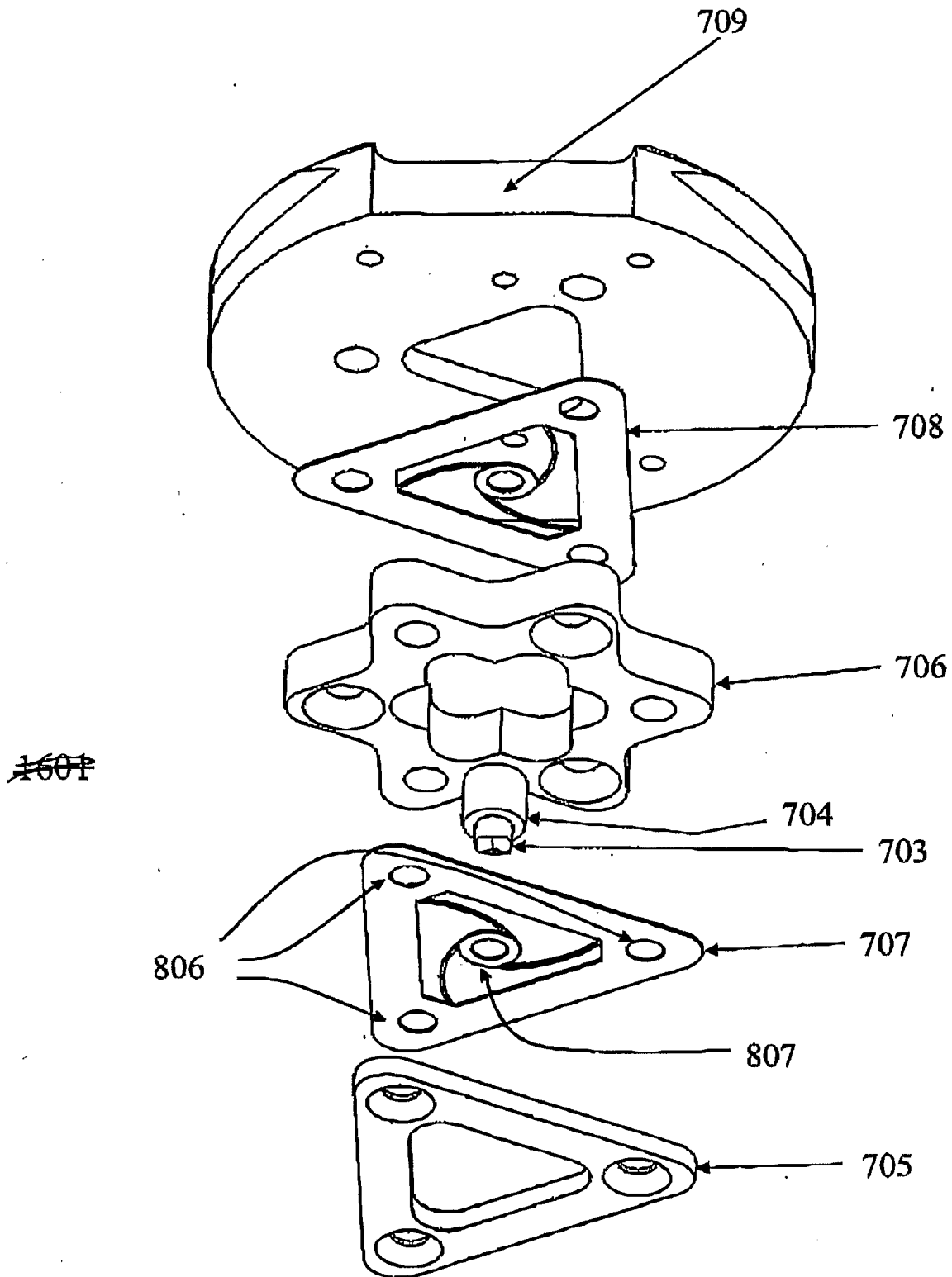
FIG. 16 Nanoindenter scheme 3 before assembly
