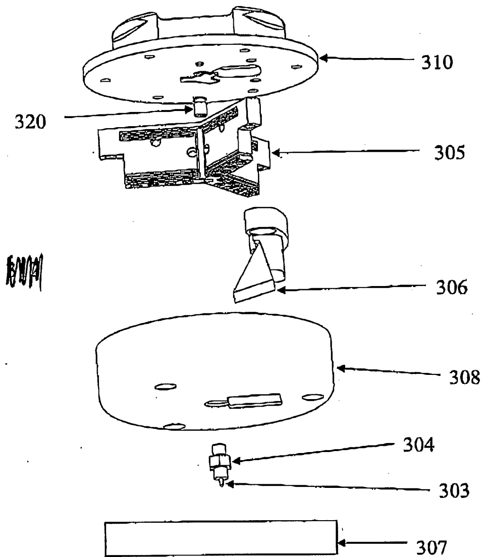
FIG. 3 Nanoindenter before assembly
