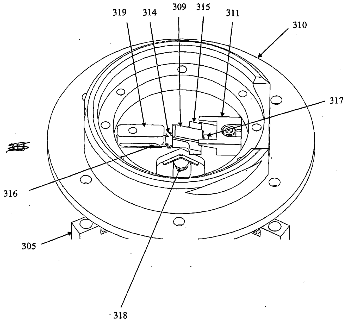
FIG. 7 Nanoindenter, optical lever detection detailed.
