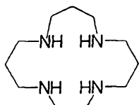
1,4,8,12-tetraaza cyclopentadecane
