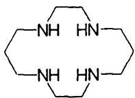
1,4,8,11-Tetraaza cyclotetradecane
