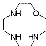
1-Oxa-4,7,10-triazacyclododecane
