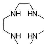
1,4,7,10-Tetraaza cyclododecane
