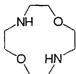
1,7-Dioxo-4,10-diazacyclododecane
