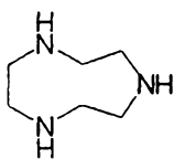
1,4,7-Triazacyclononane
