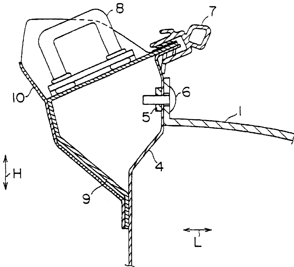
Fig. 5 PRIOR ART
