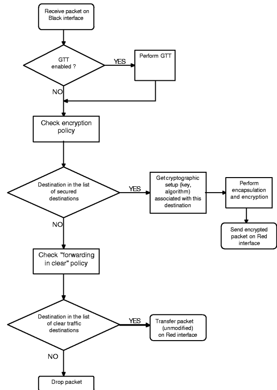
Figure 2: SVSG Encryption Flow Chart
