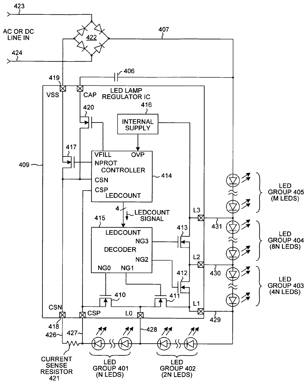
LED LAMP FIG. 14
