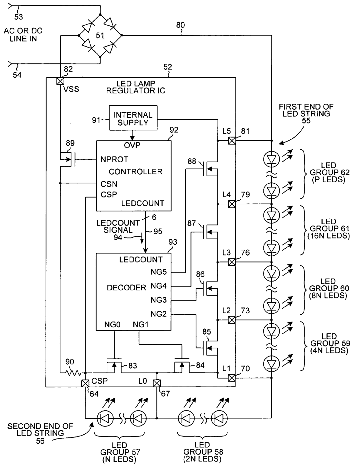
LED LAMP FIG. 4
