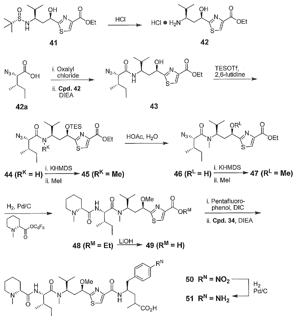
Scheme 5
