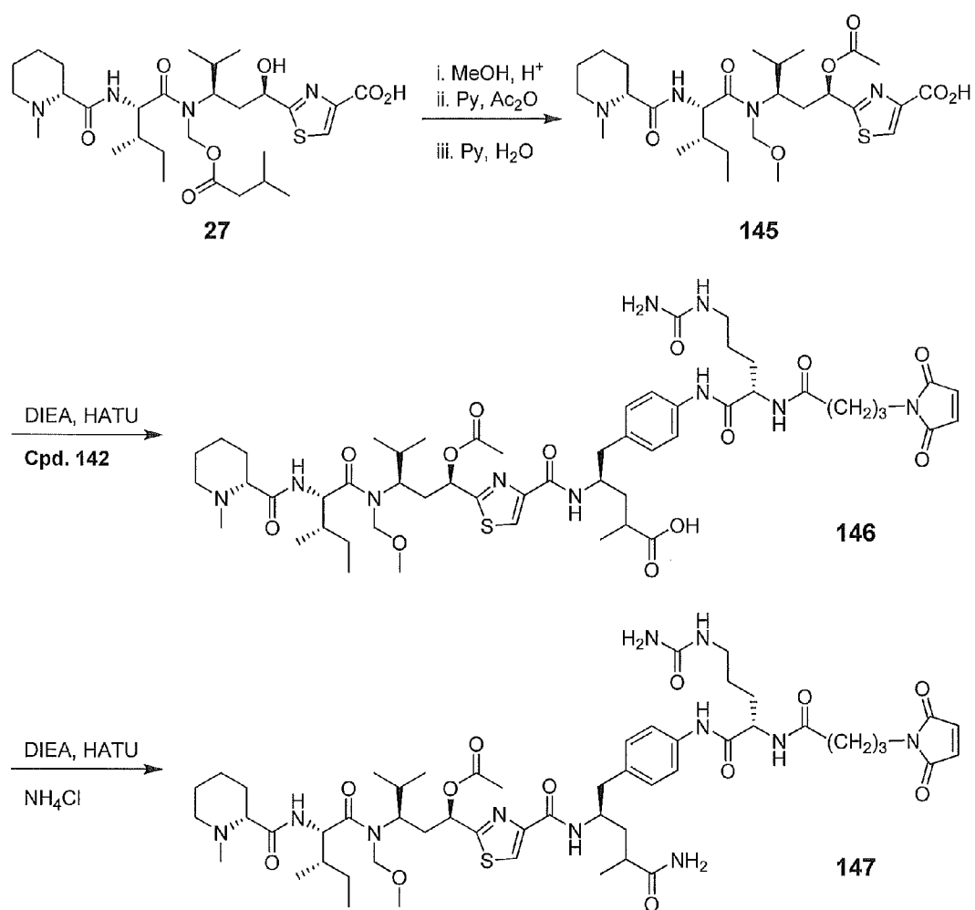
Scheme 23
