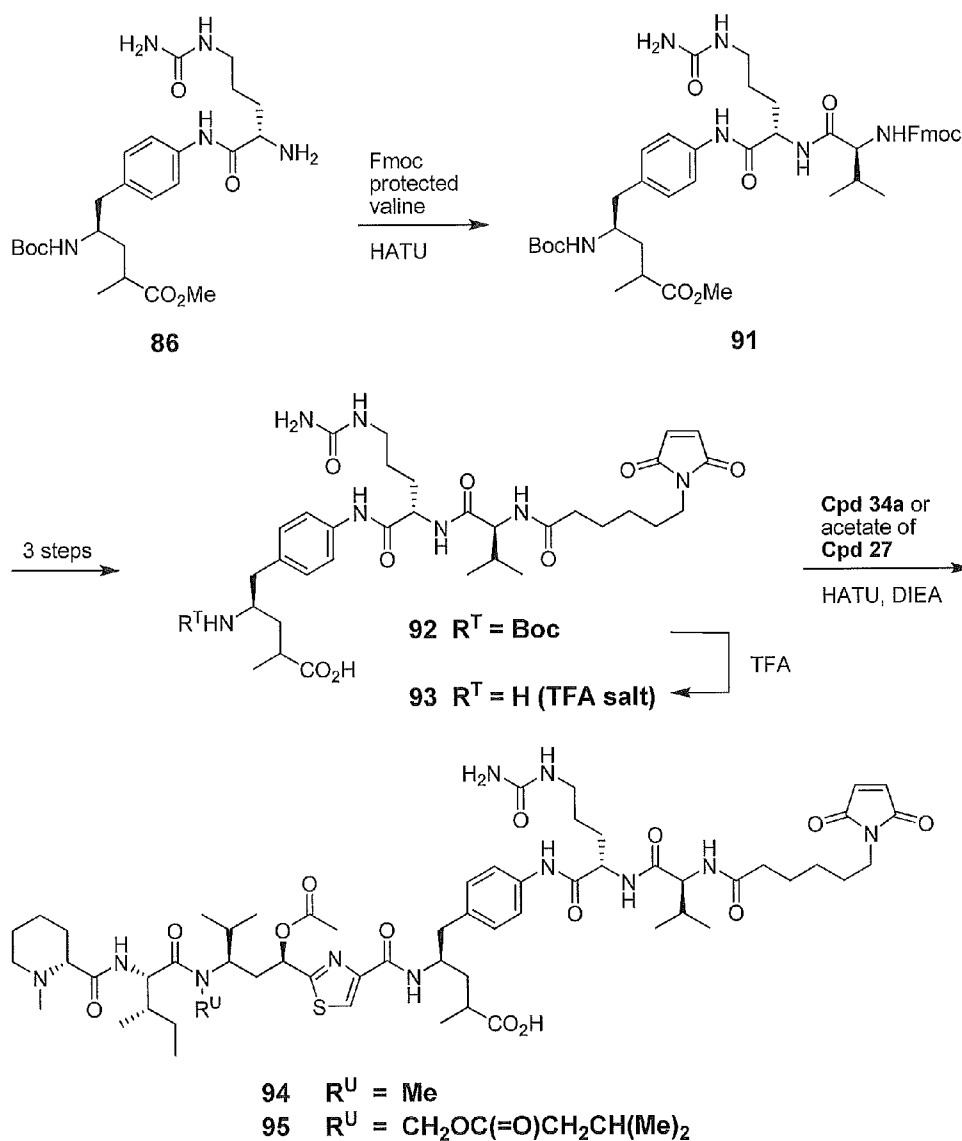
Scheme 16
