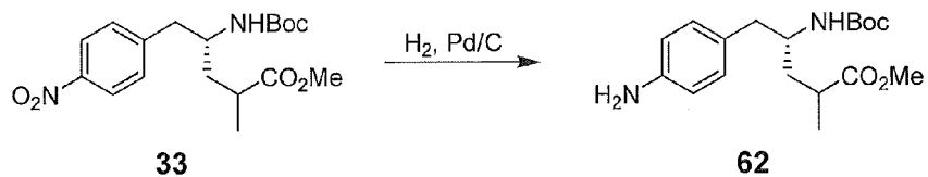
Scheme 10
