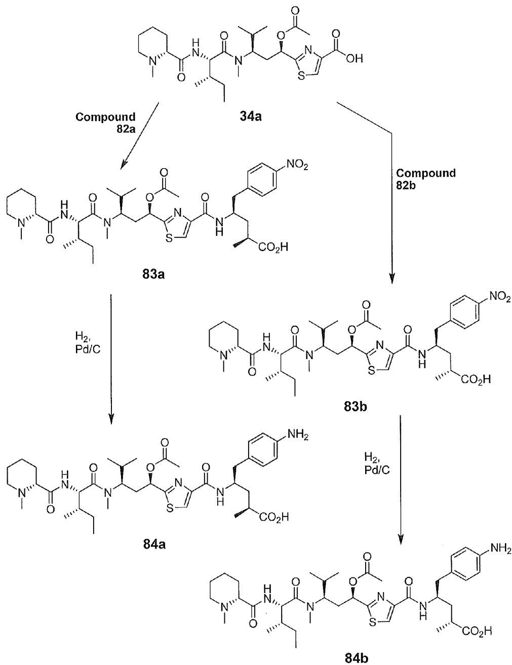
Scheme 14
