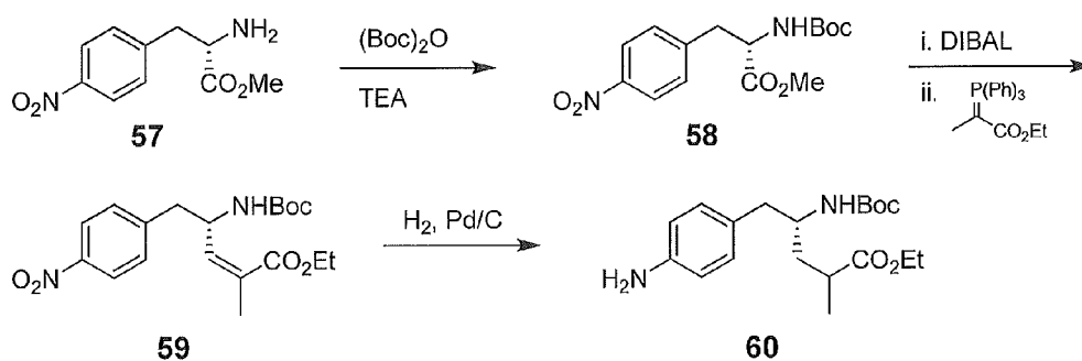
Scheme 8
