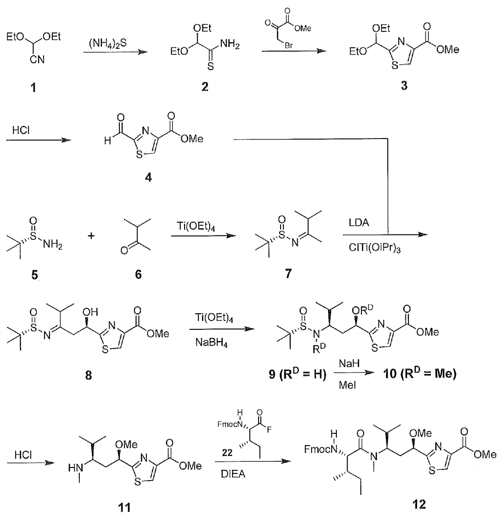
Scheme 1 (part 1 of 2)
