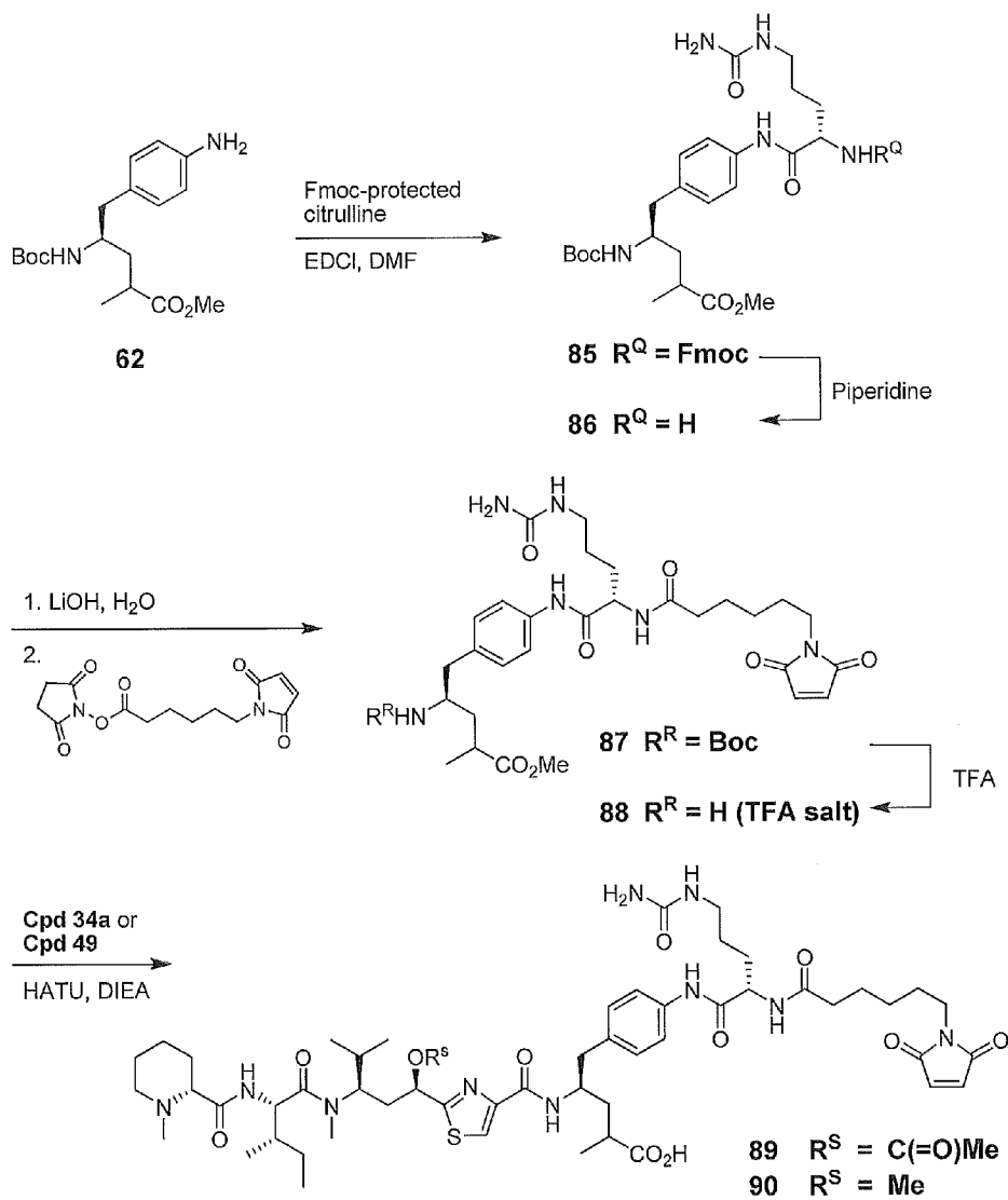
Scheme 15
