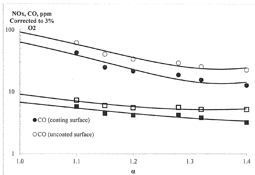
Flue gas CO and NOx corrected concentrations at different excess air ratio ( W=33\text{w/cm}^2 ).
