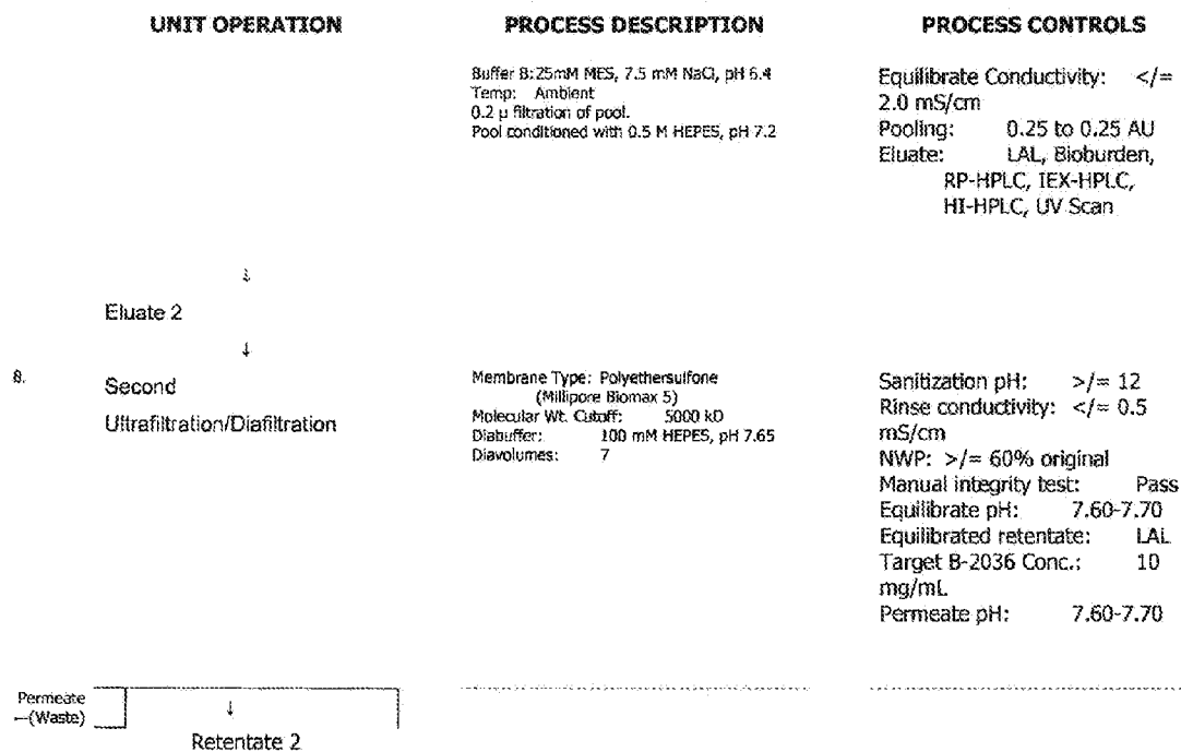
Flowchart 2 Process Flow Diagram for Recovery &amp; Purification to B-2036 (Bulk Intermediate)
