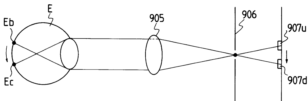
FIG. 13 PRIOR ART
