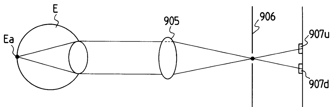
FIG. 12 PRIOR ART
