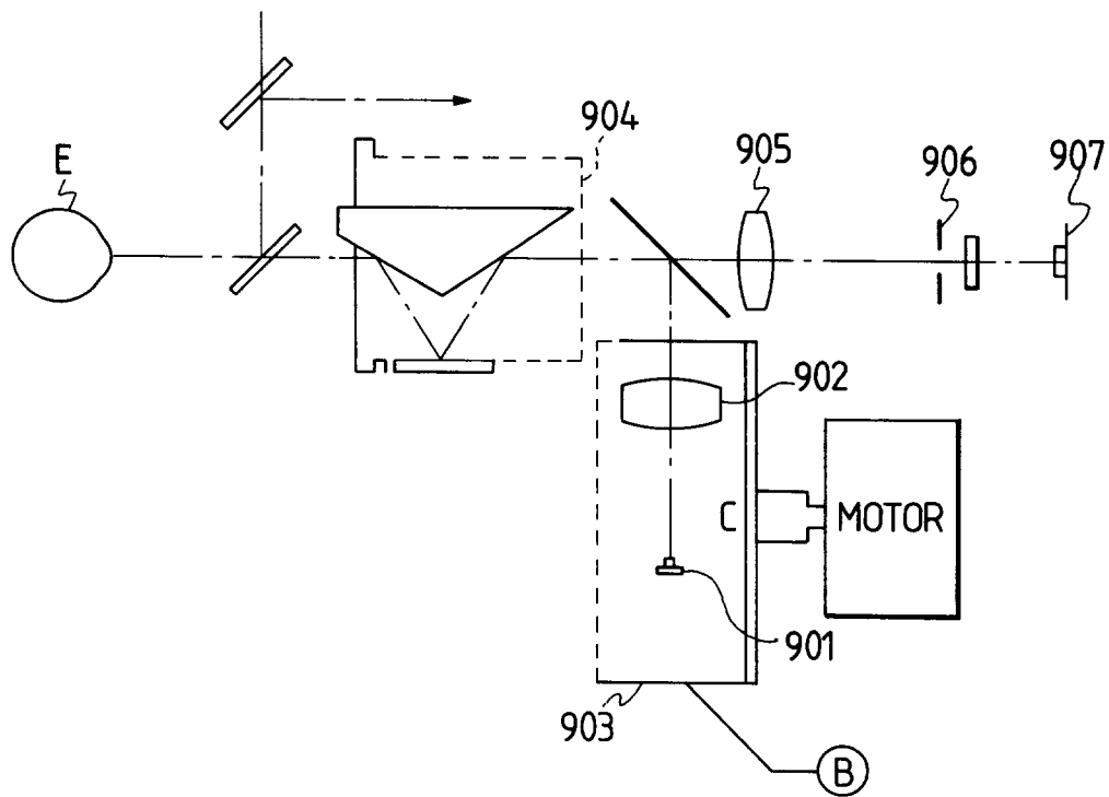
FIG. 11 PRIOR ART
