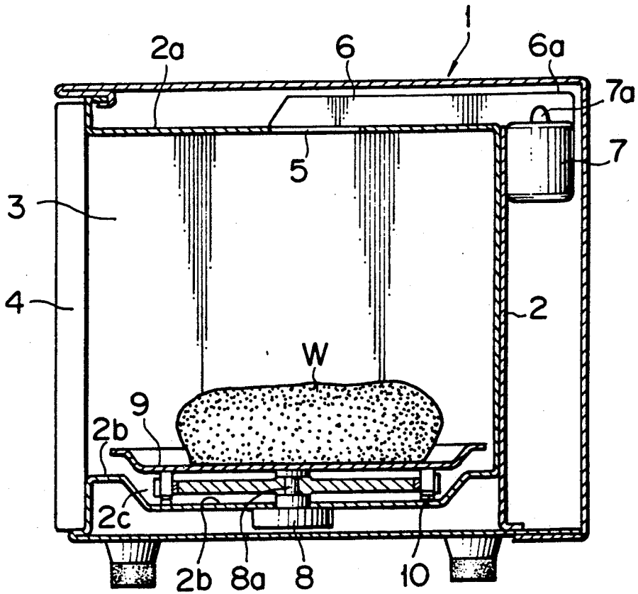
FIG. 8 PRIOR ART
