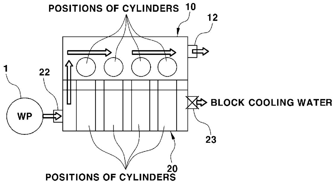
FIG. 2 (RELATED ART)
