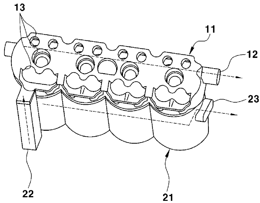
FIG. 1 (RELATED ART)
