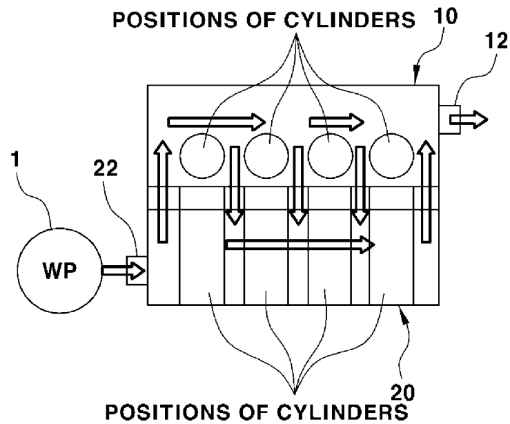
FIG. 3 (RELATED ART)
