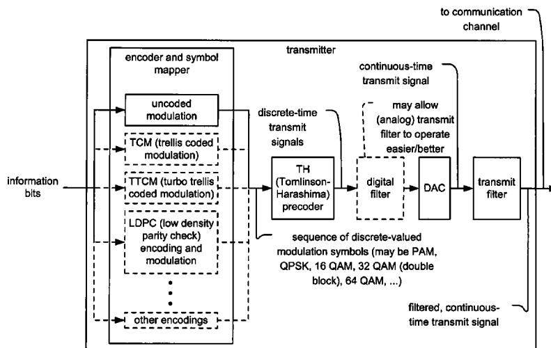
ZEB modulation communication transmitter including various forms of encoding and symbol mapping and TH precoding
