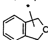
1,3-dihydroisobenzofuranyl; phthalanyl (1.4.6)
