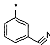
(2.0.4)
