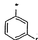
(2.0.8)
