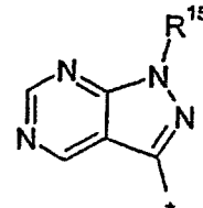
1H-pyrazolo[3,4-d]- pyrimidinyl (1.4.23)
