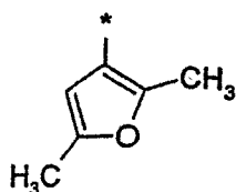
(2.0.25)
