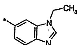
(2.0.66)
