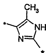
(3.0.18)
