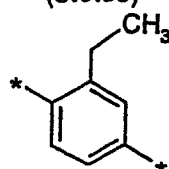
(3.0.33)
