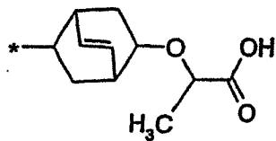
(1.5.34)
