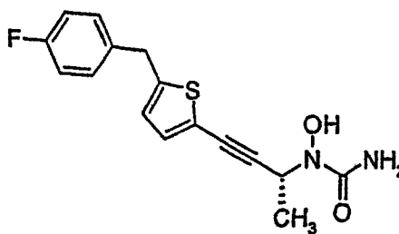
ABT-761
