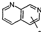
pyridopyridinyl (1.4.26)
