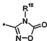
1,2,4-oxadiazol- 5-on-3-yl (1.1.21)
