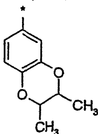
(1.8.13)
