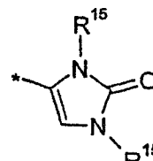
imidazolidin-2-on-4-yl (1.1.17)
