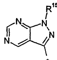
1H-pyrazolo[3,4-d]- pyrimidinyl (5.0.23)
