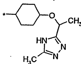
(1.5.50)
