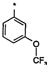
(1.8.10)
