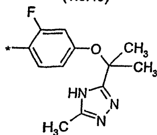
(1.5.52)
