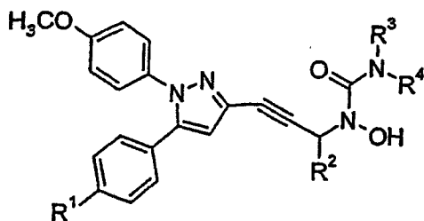
(5.2.4)
