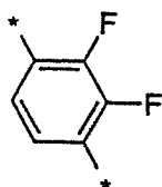
(2.5.2)
