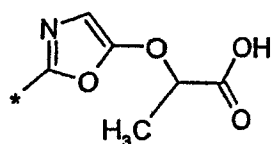
(1.5.40)
