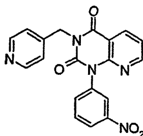
RS-25,344
