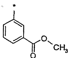
(2.0.38)
