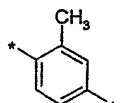
(2.5.34)
