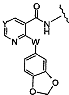
(1.0.15)
