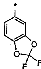
(2.0.12)
