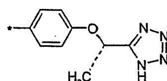
(1.5.15)
