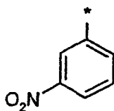
(1.8.5)
