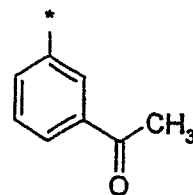
(2.0.72)
