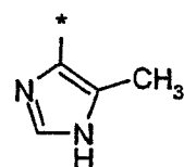
(2.0.35)
