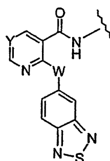
(1.0.17)
