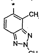
(1.8.20)
