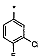
(1.8.3)
