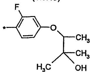
(1.5.40)
