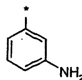
(2.0.24)
