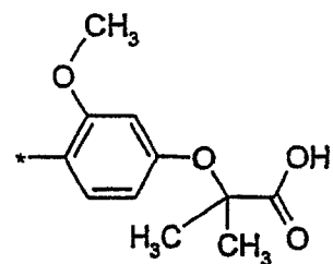
(1.5.6)
