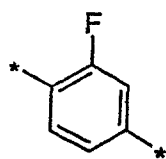
(3.0.1)
