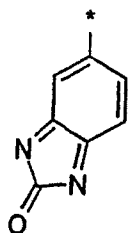
(2.0.18)
