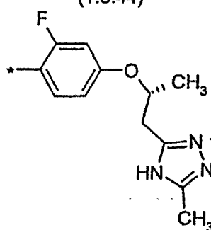
(1.5.47)
