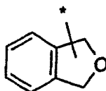
1,3-dihydroisobenzofuranyl; phthalanyl (5.0.6)
