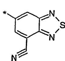
(2.0.17)
