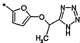
(1.5.31)
