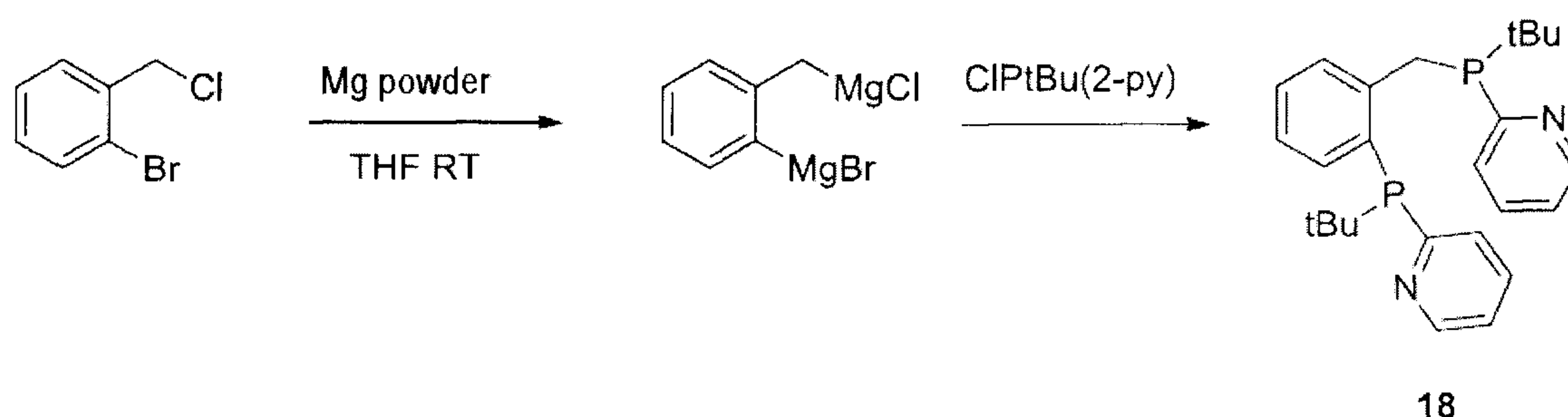
Scheme 3: Synthesis of compound 18
