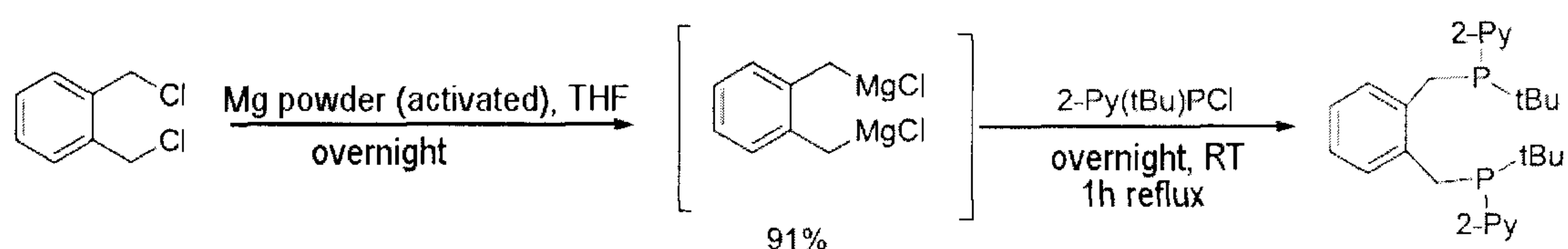
Scheme 2: Synthesis of compound 1
