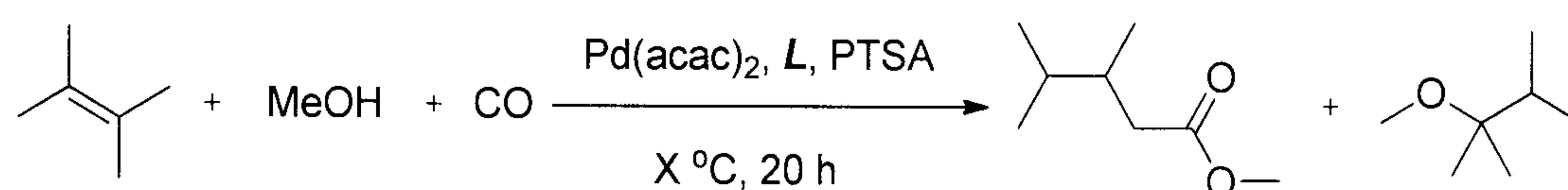
Scheme 5: Methoxycarbonylation of tetramethylethylene.
