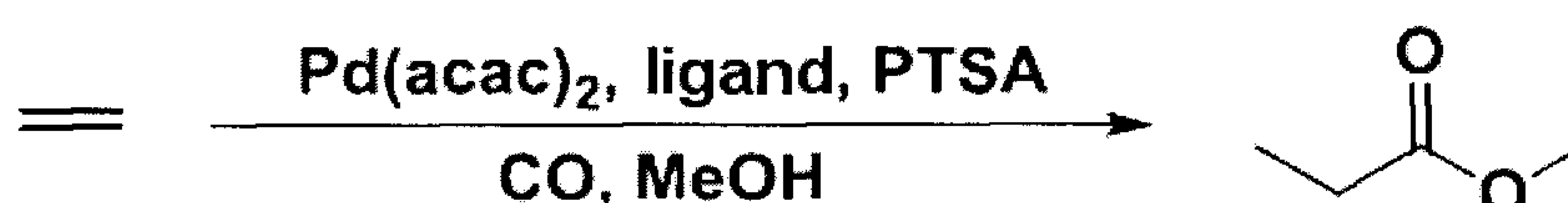
Scheme 4: Methoxycarbonylation of ethene.
