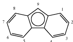
Fluorenyl
