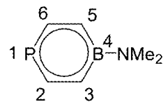
4-dimethylamino- 1,4-phosphaboratabenzene
