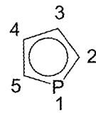
phosphacyclopentadienyl
