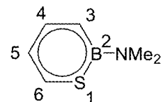
2-dimethylamino- 1,2-azaboratabenzene
