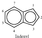
Indenyl
