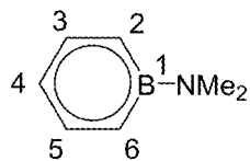
1-dimethylamino- boratabenzene
