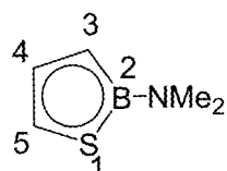
2-dimethylamino- 1,2-thiaborollide
