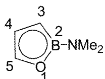
2-dimethylamino- 1,2-oxaborollide
