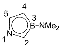
3-dimethylamino- 1,3-azaborollide
