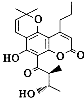
(±)-8b
