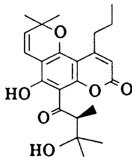
(±)-14b
