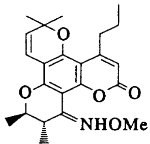
(±)-19b
