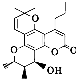
(-)-Calanolide B
