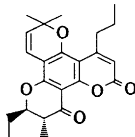
(±)-15c
