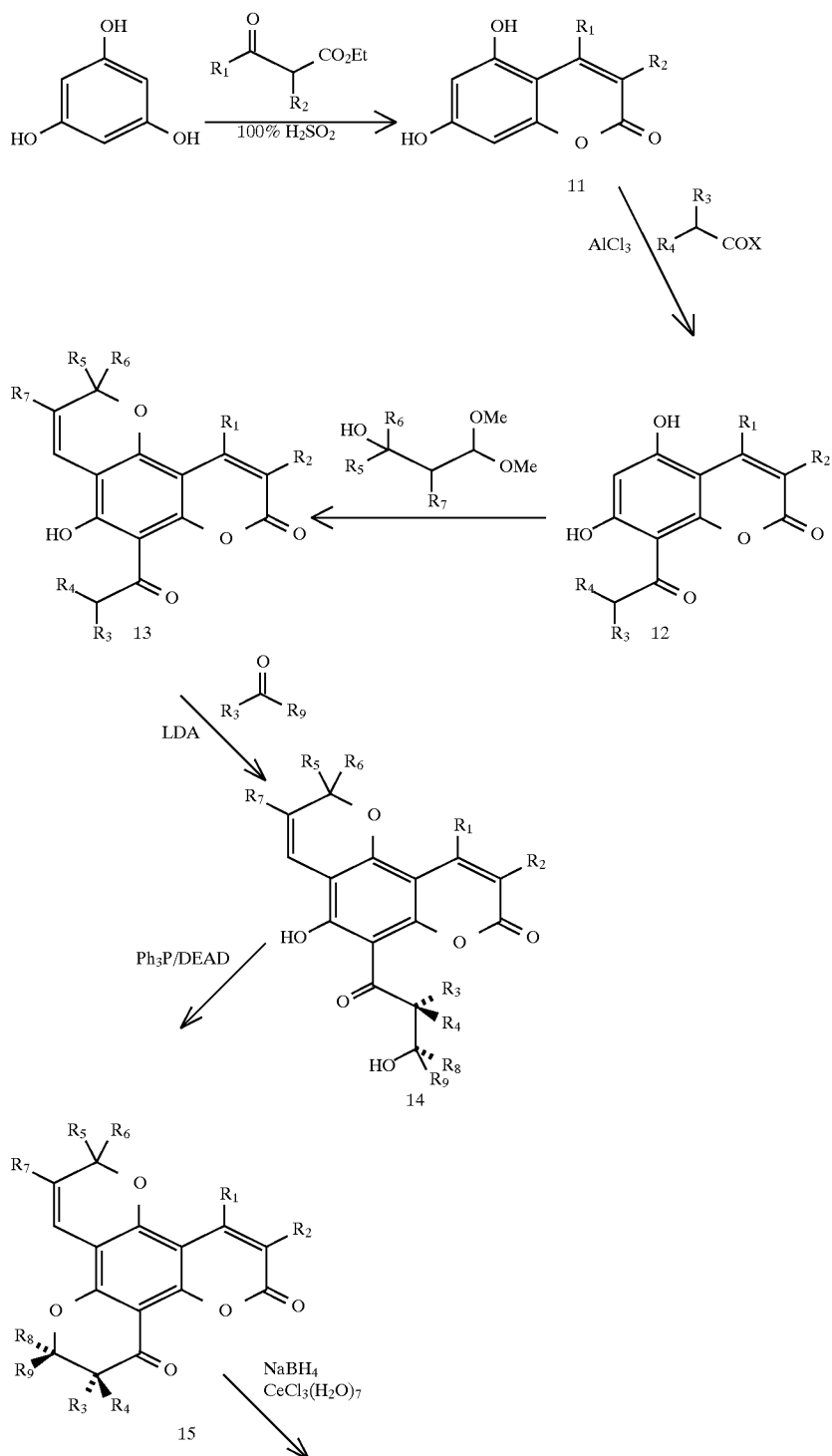
Scheme V
