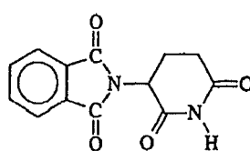
thalidomide
