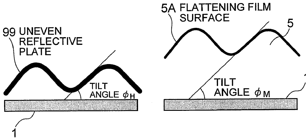
DEFINITION OF TILT ANGLE
