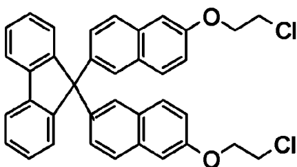
Compound 4
