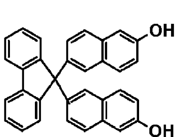
Compound 5
