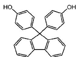
Comparative compound 2
