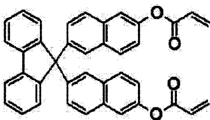
Compound 11
