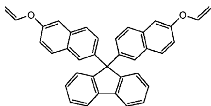
Compound 1
