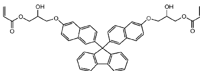
Comparative compound 5
