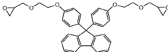
Comparative compound 4
