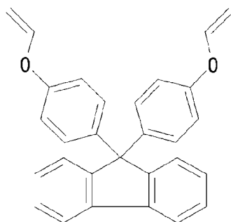
Compound 3
