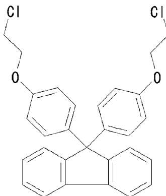
Compound 10
