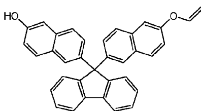
Compound 2
