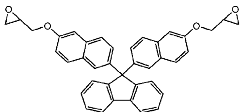
Comparative compound 3
