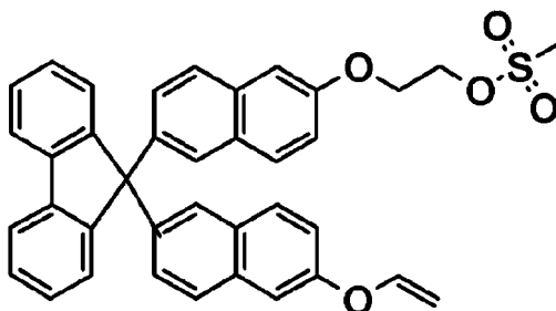
Compound 7
