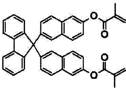
Compound 12
