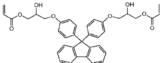
Comparative compound 6
