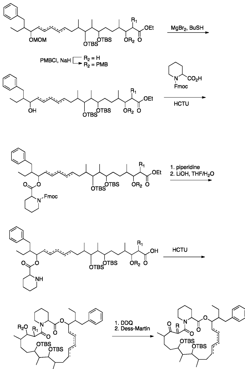
Scheme 4: Macrocyclization
