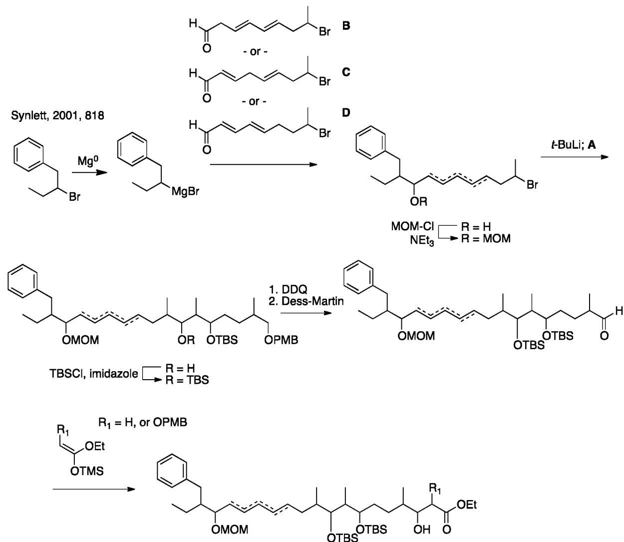
Scheme 1: Synthesis of a Linear Intermediate
