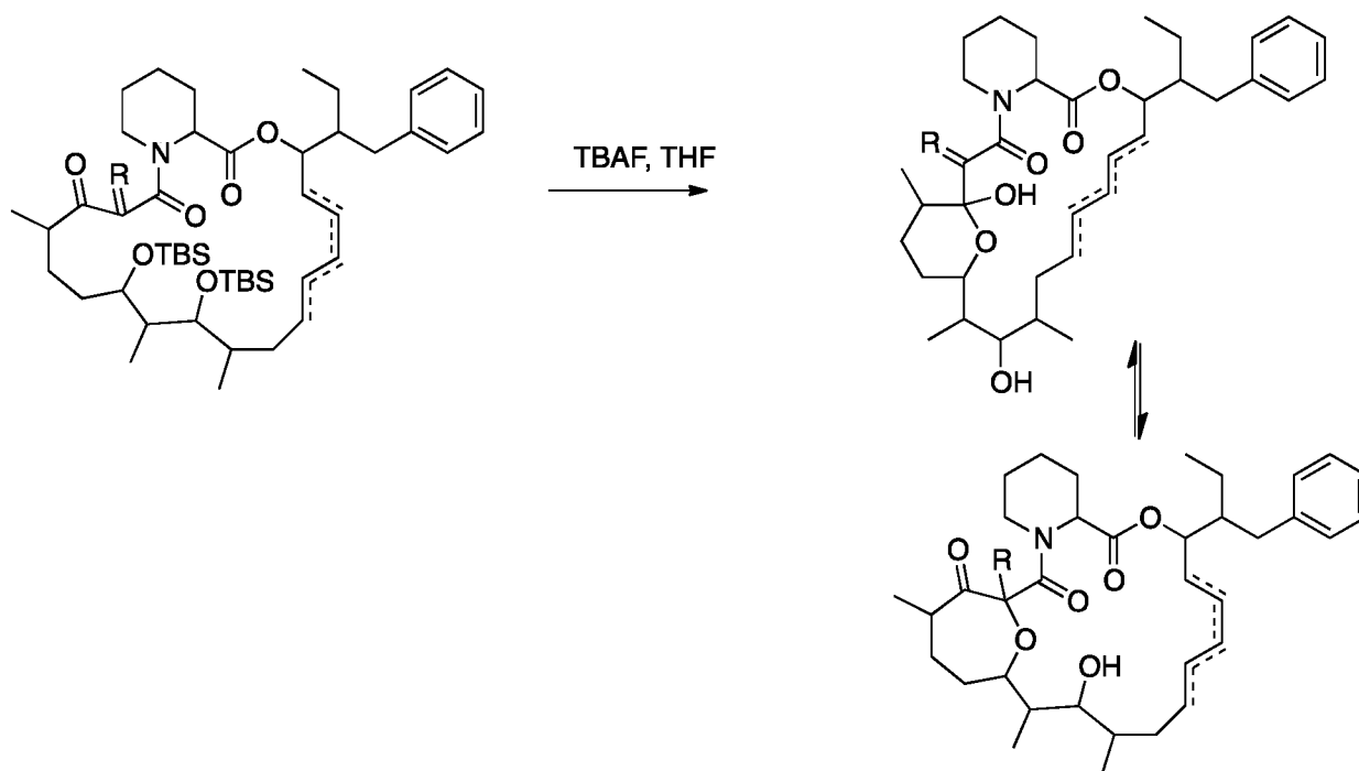
Scheme 5: Cyclization to Compounds of Formula I
