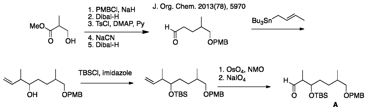
Scheme 2: Synthesis of Intermediate A
