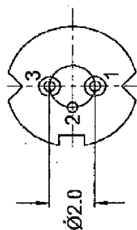
Bottom View
