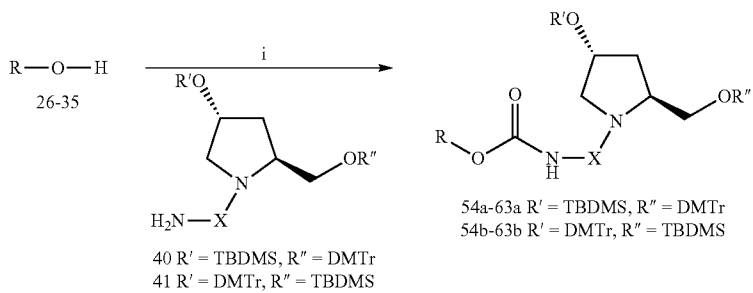
Scheme 7 a
