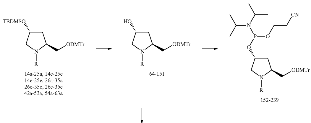
Scheme 8 a
