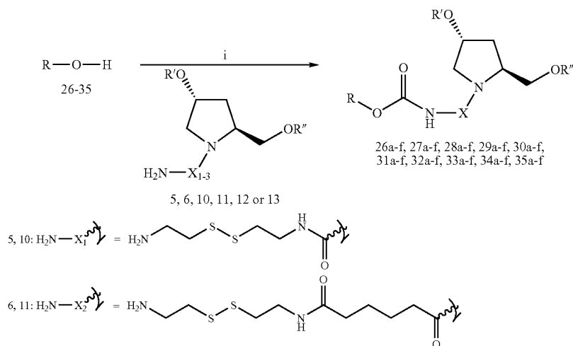
Scheme 4 a
