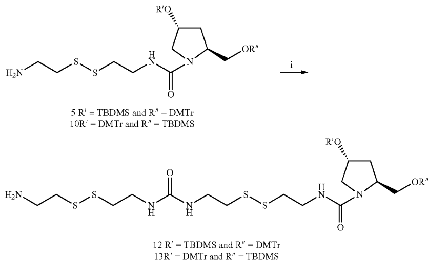
Scheme 2 a
