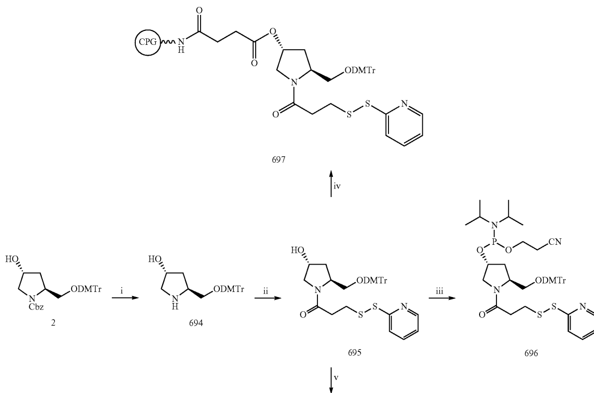
Scheme 9 a
