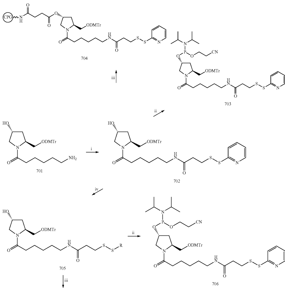
Scheme 10 2
