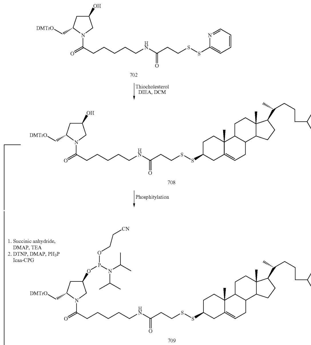
Scheme 11: Synthesis of Thiocholesterol-Hydroxyprolinol Building Blocks containing a disulfide linkage
