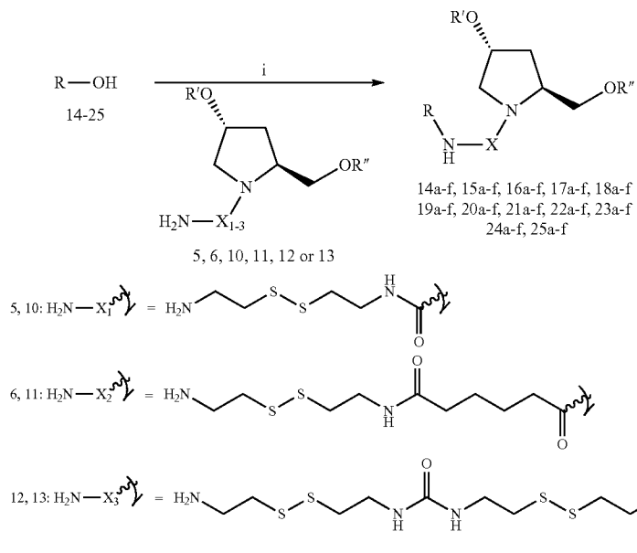
Scheme 3 a
