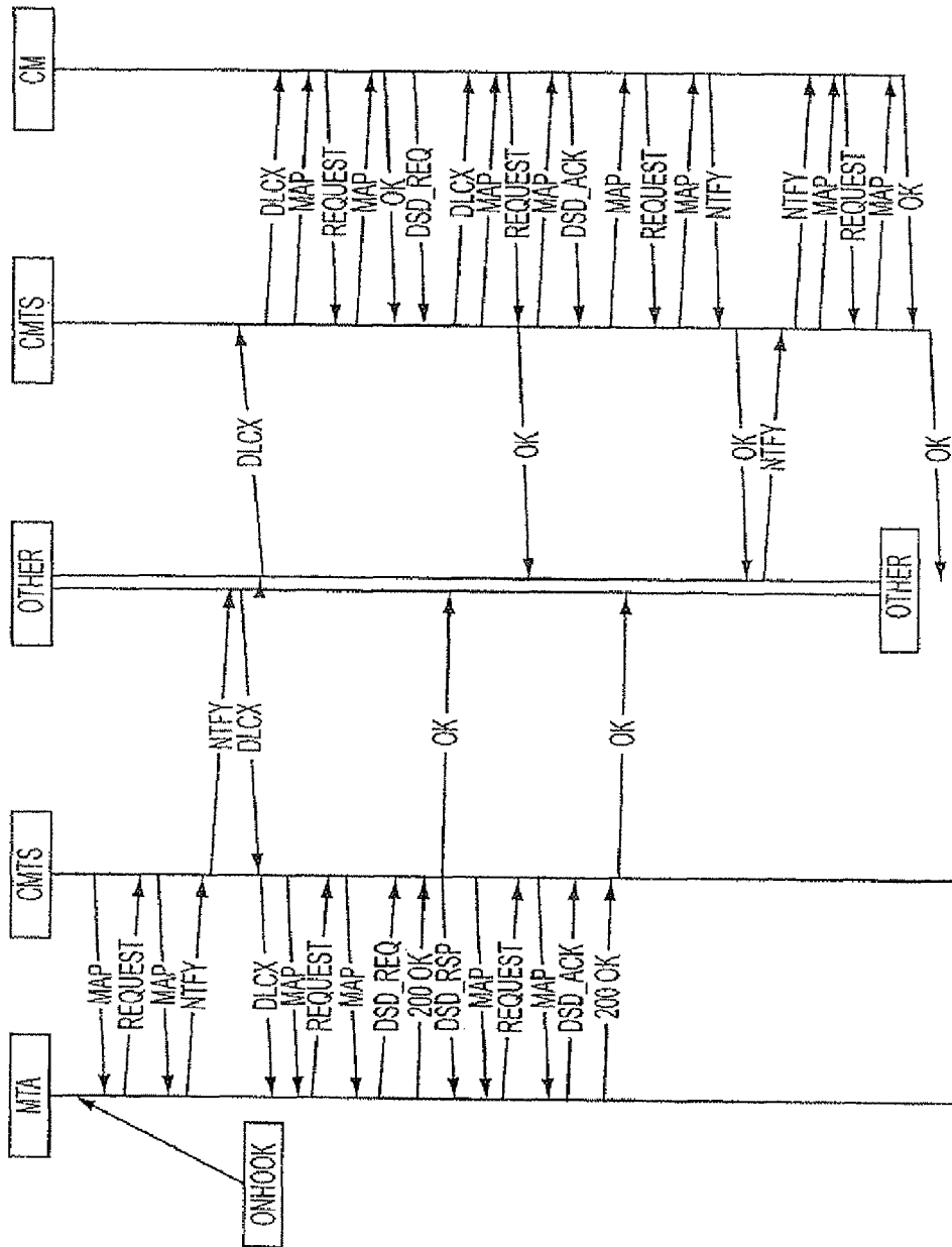
FIG. 13 RELATED ART
