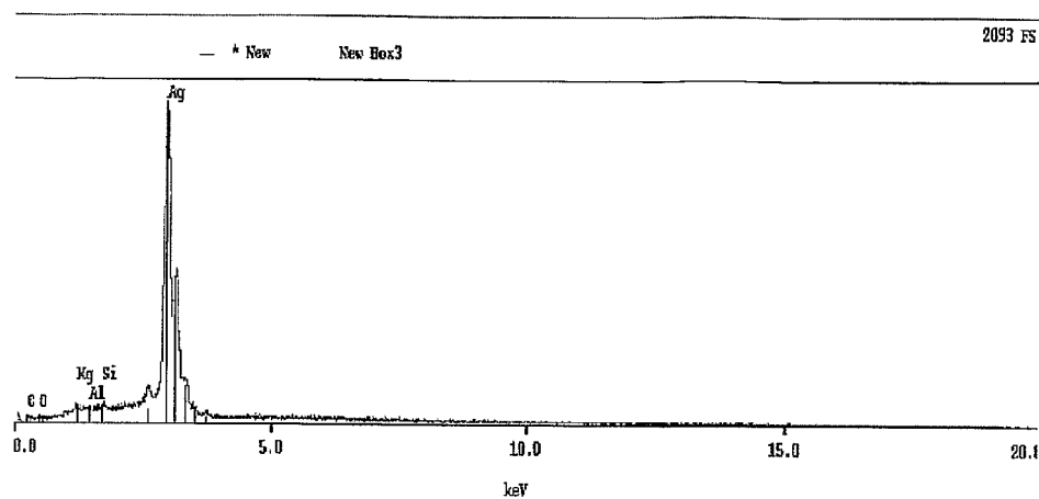
EDS Elemental Analysis of New Electrode Box 3
