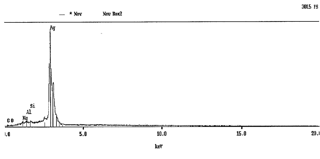
EDS Elemental Analysis of New electrode Box 2
