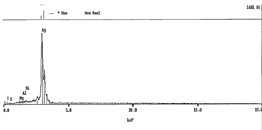
EDS Elemental Analysis of New Electrode Box 1
