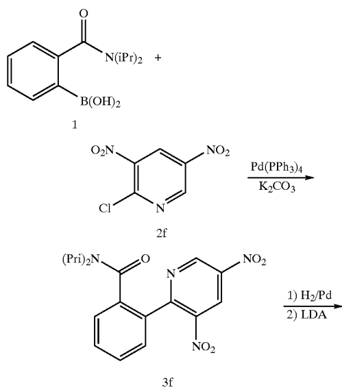
Scheme 2-5. Synthesis of Aminoazaphenanthridone 4f.
