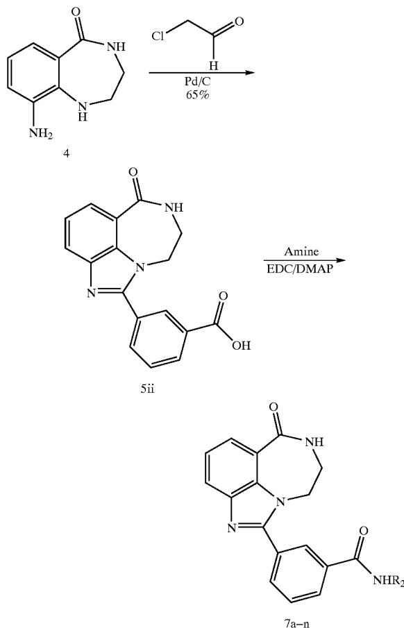
Scheme 4-4. General Synthesis of amides 7a-n.
