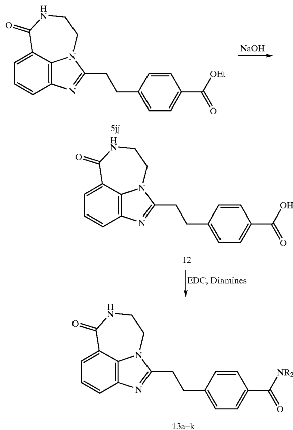
Scheme 7-4. Synthesis of amides 13a-k.
