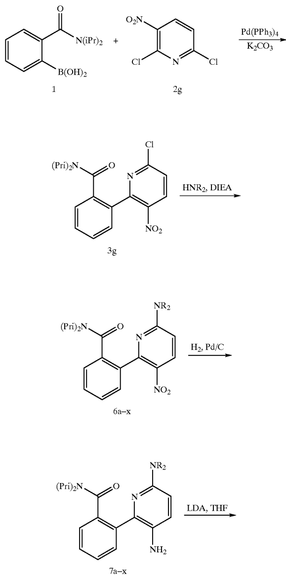
Scheme 4-5. General Scheme for synthesis of azaphenanthridone amines 4h-x.
