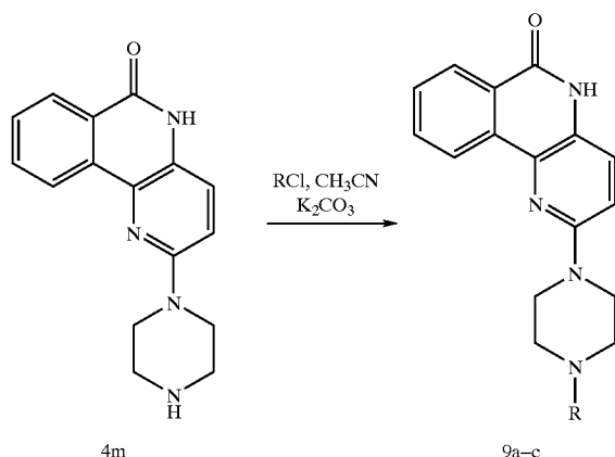
Scheme 6-5. Synthesis of amines 9a-c.
