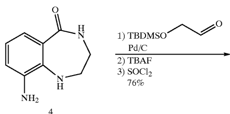
Scheme 3-4a. Alternative Synthesis of imidazobenzodiazepine amines 6a-kk.
