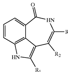
Scheme 1-3
