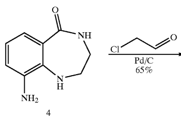
Scheme 3-4 Synthesis of imidazobenzodiazepine amines 6a-dd.
