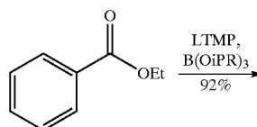
Scheme 9-5. Alternate synthesis of amines 4a-x.
