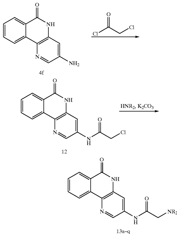
Scheme 8-5. Amide derivatives of aniline 4f.
