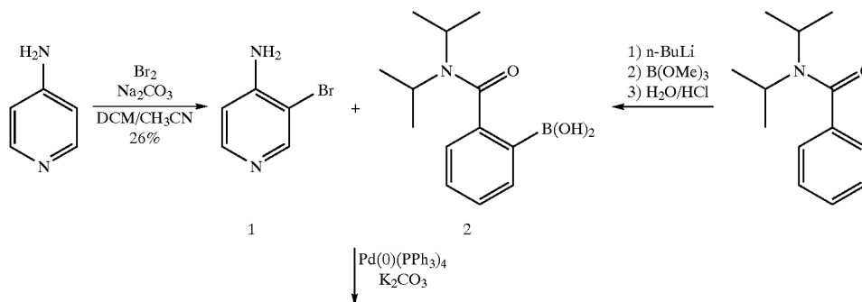
Scheme 1-6
