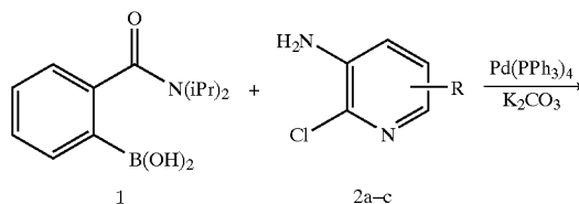
Scheme 1-5. General Scheme for synthesis of azaphenanthridones 4a-c.
