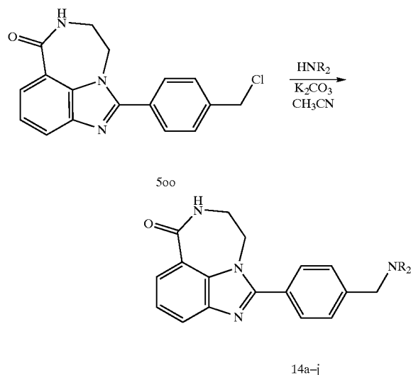
Scheme 8-4. Synthesis of amides 14a-j.
