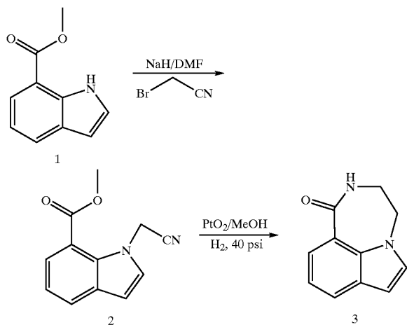
Scheme 1-8
