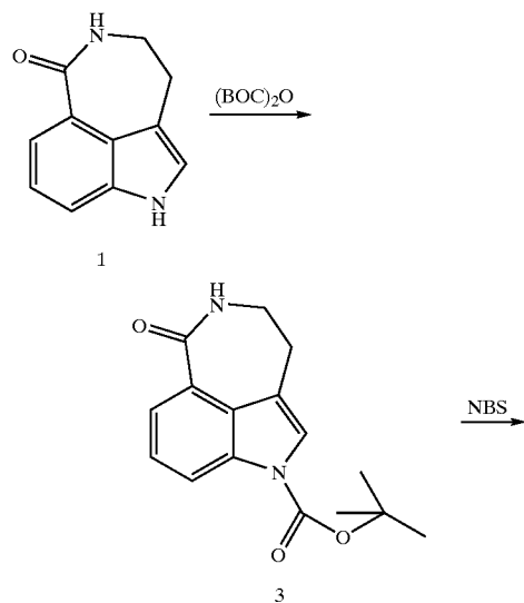
Scheme 2-3
