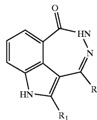
Scheme 1-1
