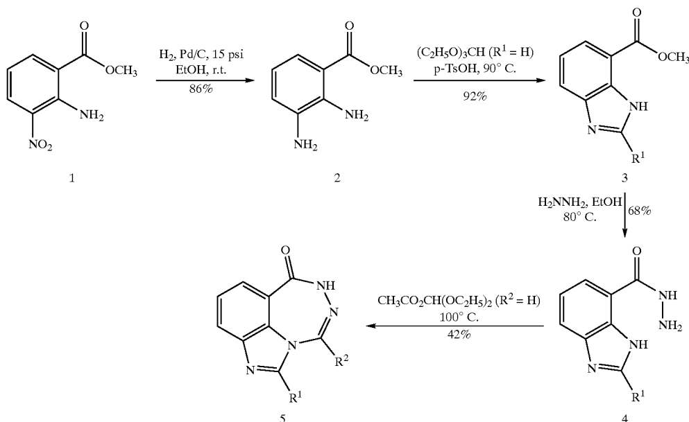
Scheme 1-7 Synthesis of Imidazolobenz-1,3,4-triazepin-5-one
