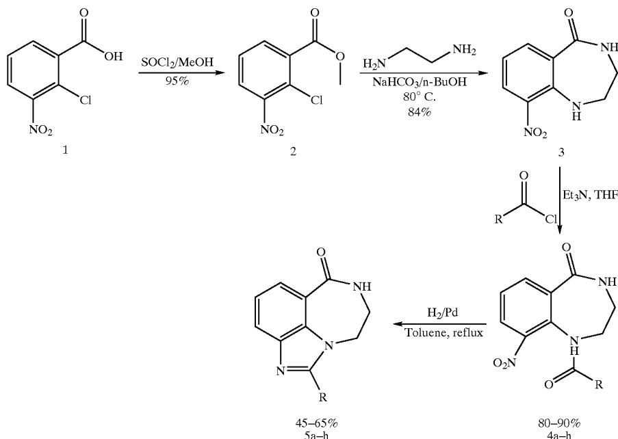
Scheme 1-4. General Synthesis of imidazo benzodiazepines:
