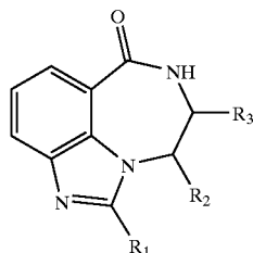
Scheme 1-4. General Synthesis of imidazo benzodiazepines:
