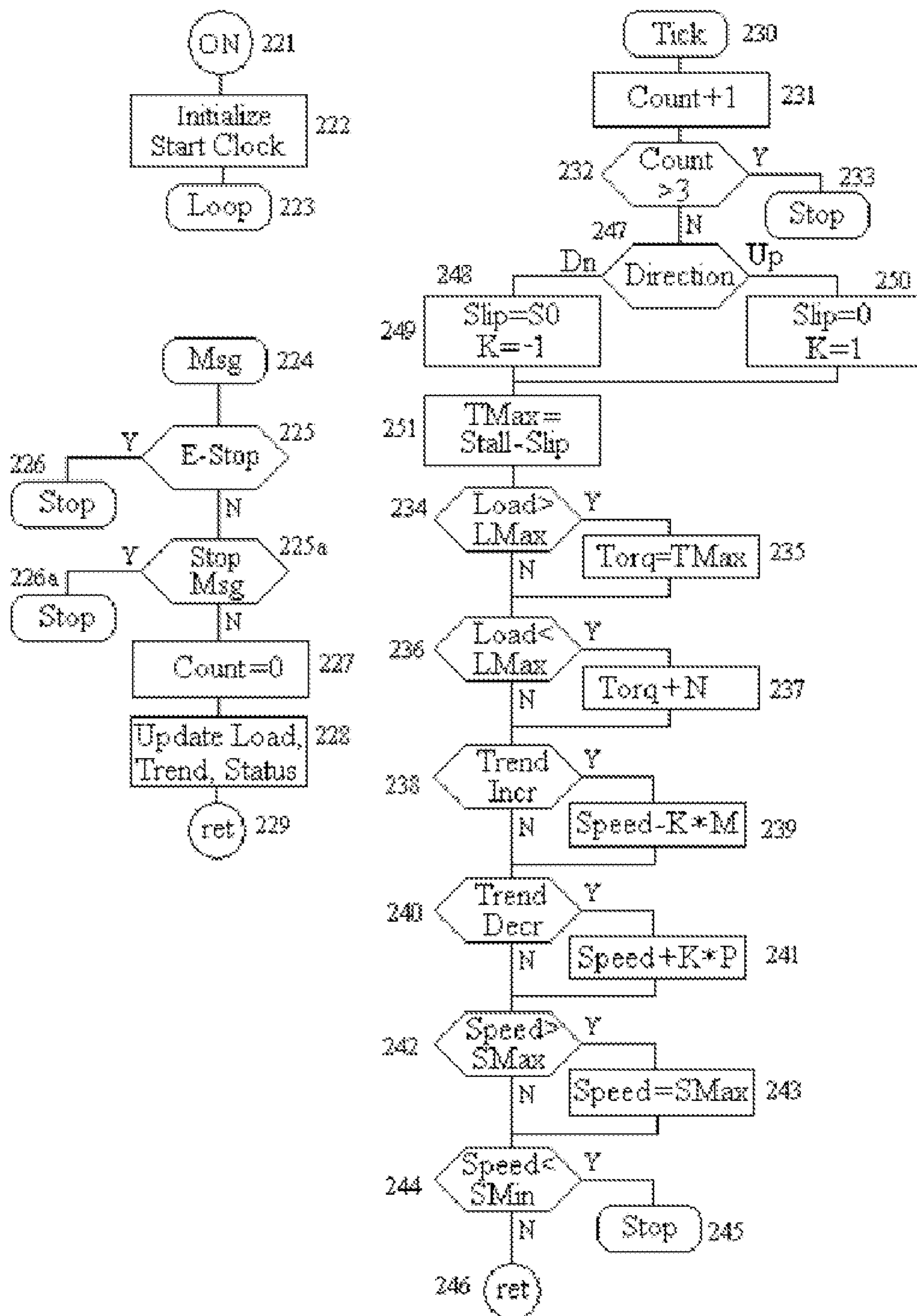
Fig 9 Receiver Logic
