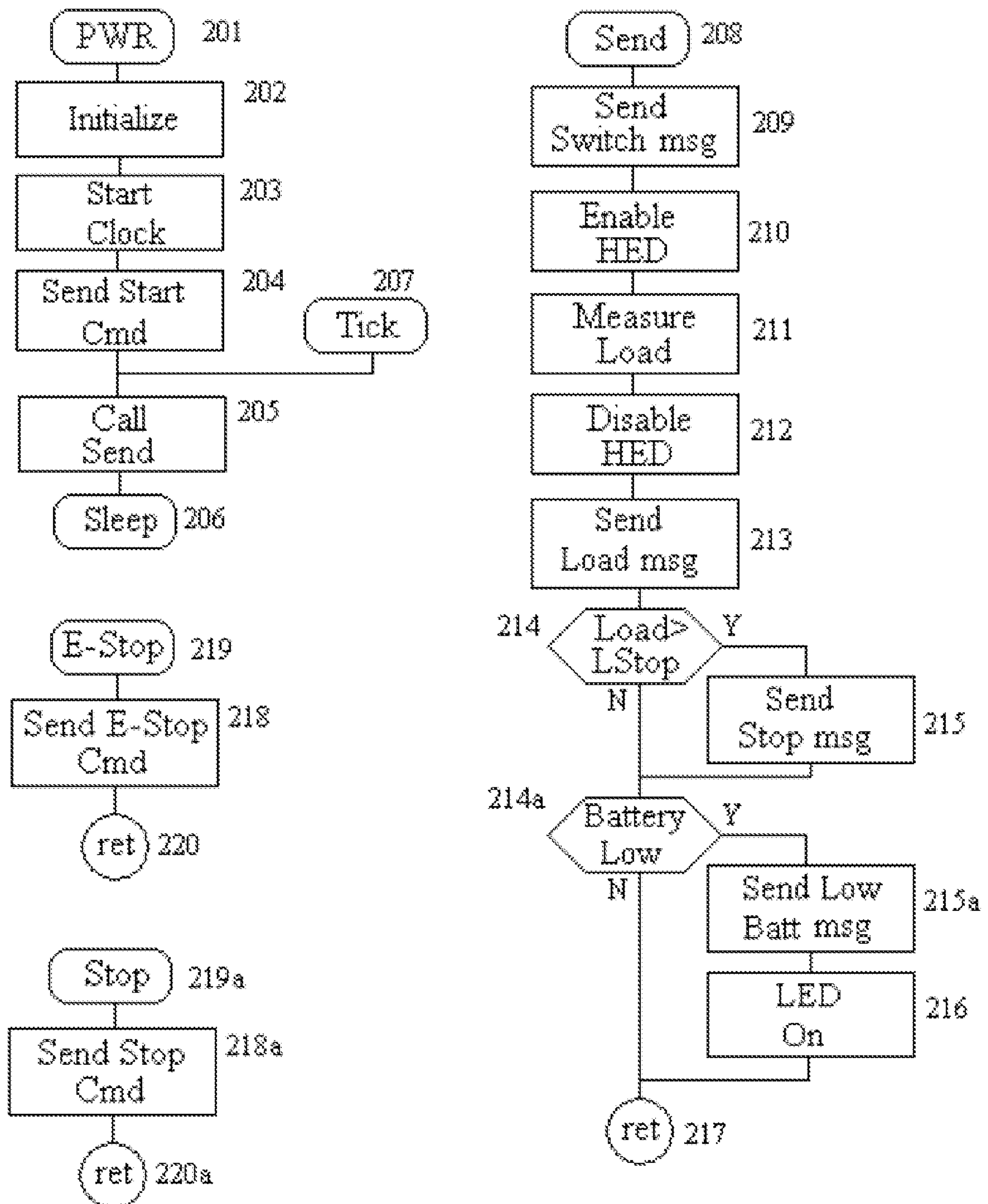
Fig 8 Sender Logic
