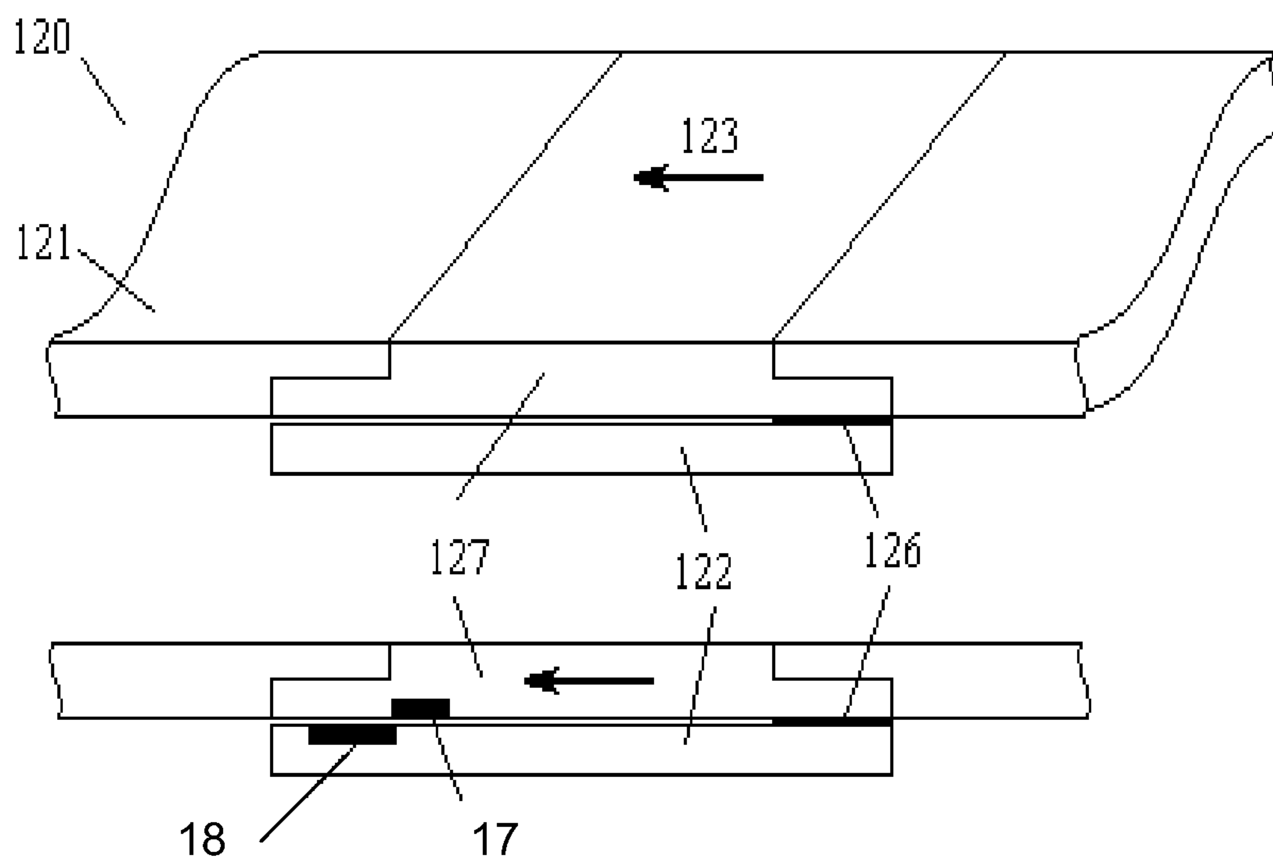
Fig 2c Sensor
