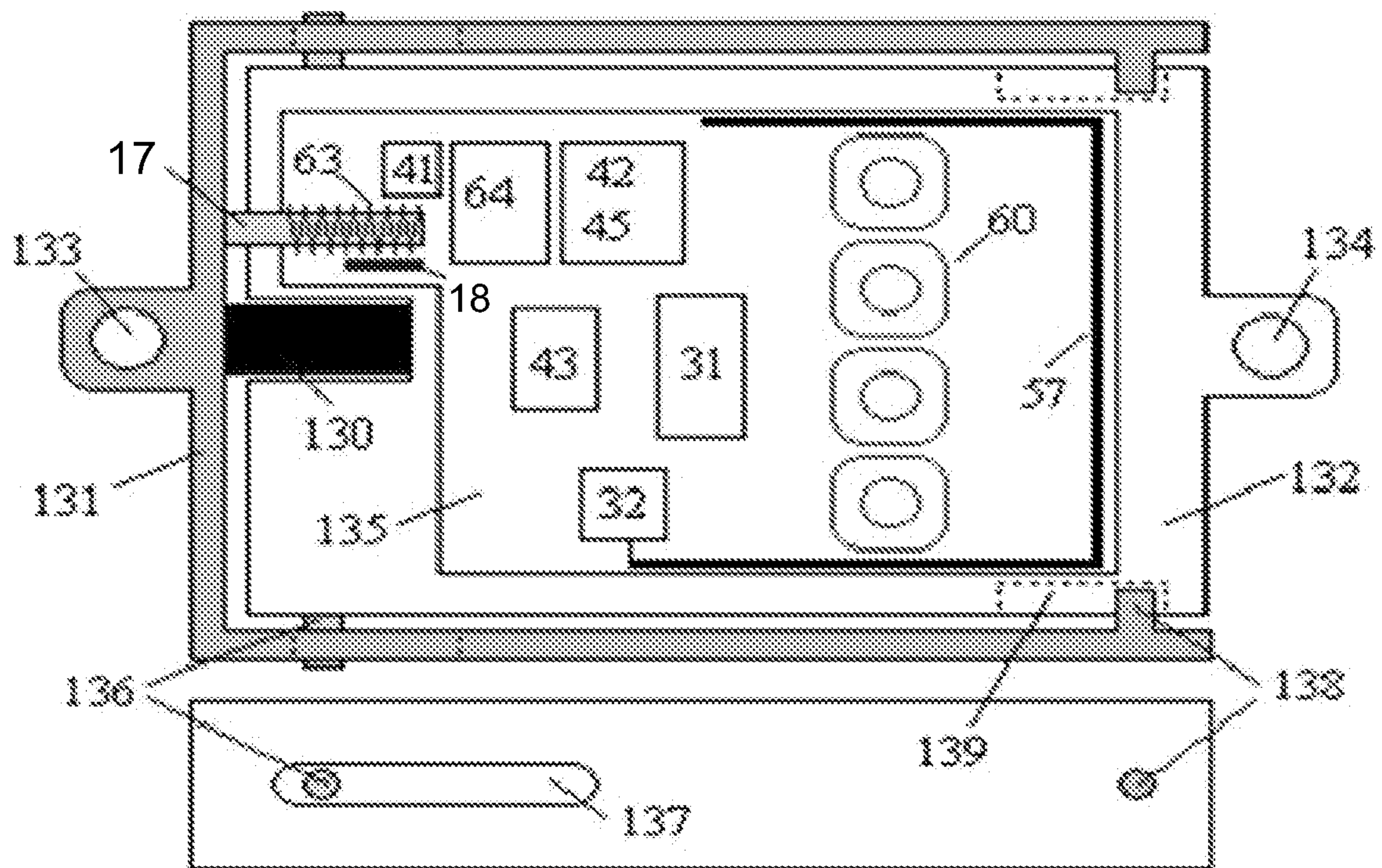
Fig 2d Sensor
