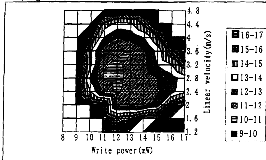
FIGURE 28 Ag5Sn6Sb66Te23
