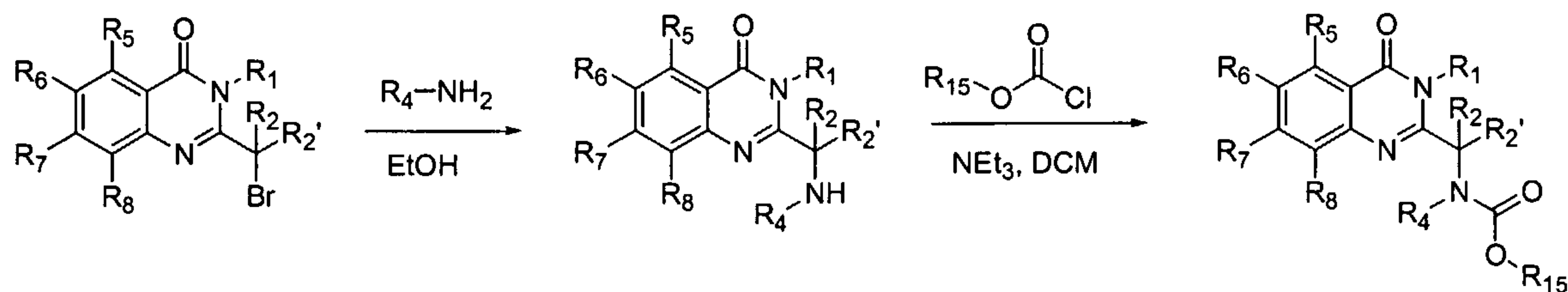
Figure 5c: Urea Synthesis
