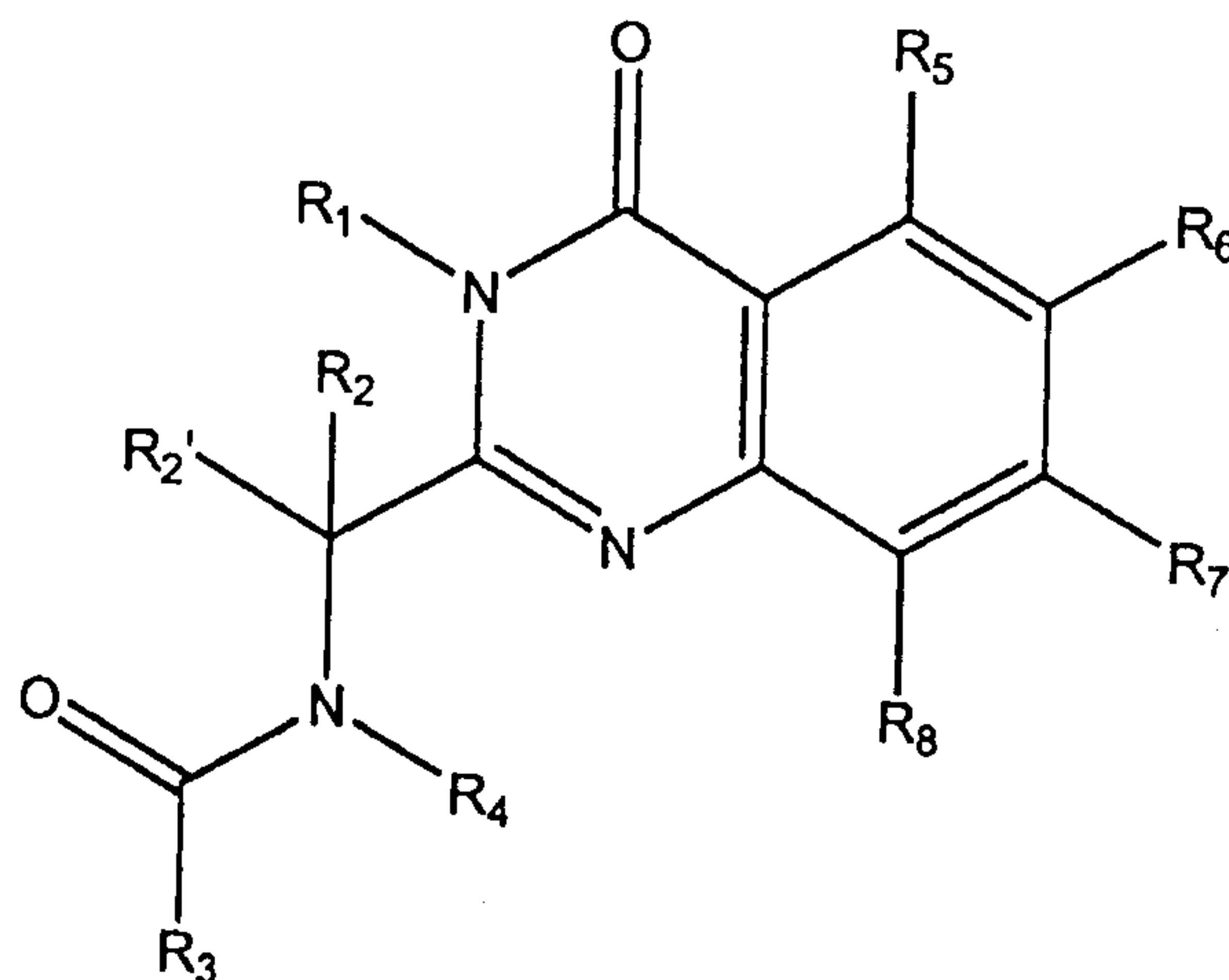
Formula 1a
