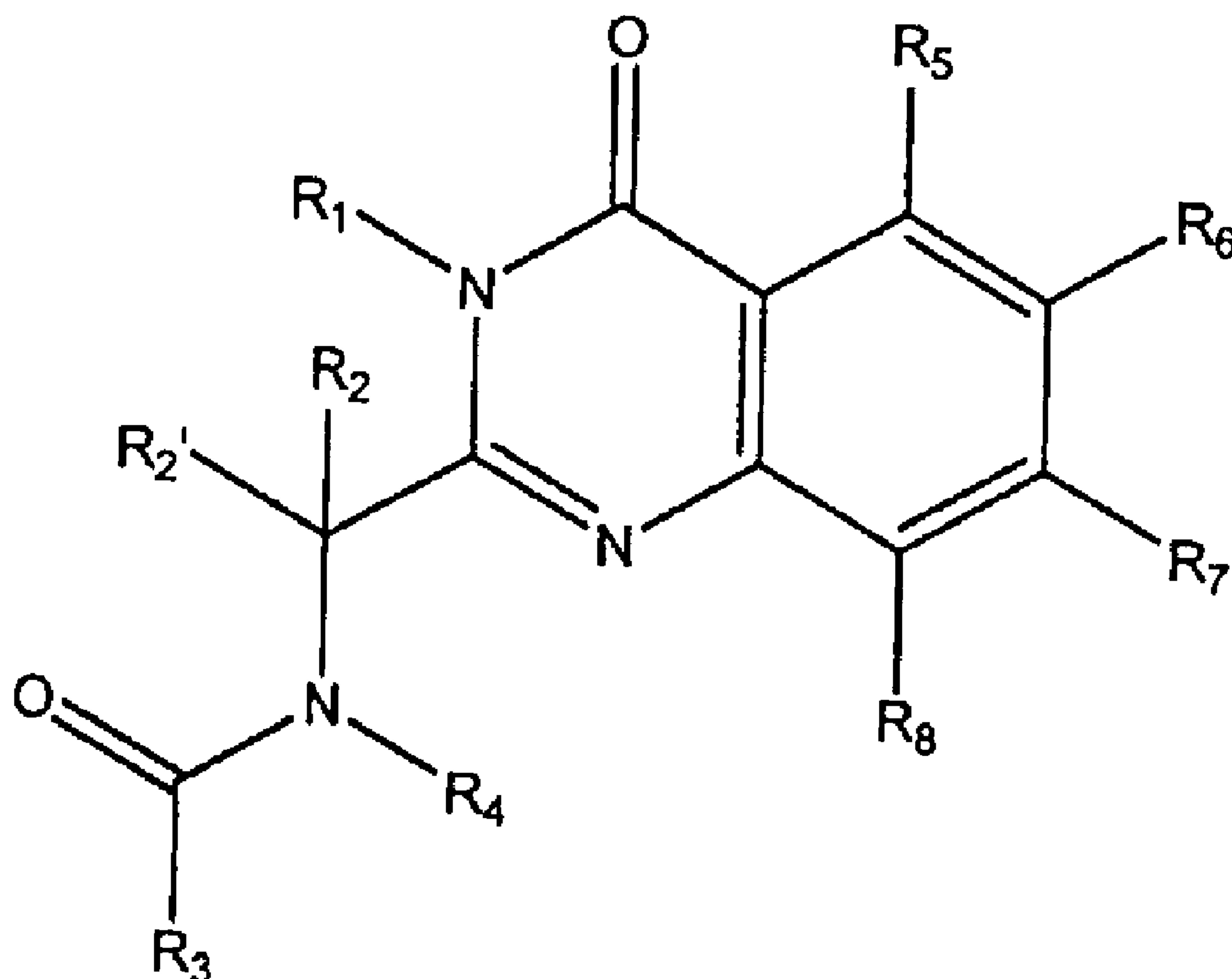
Formula 1a
