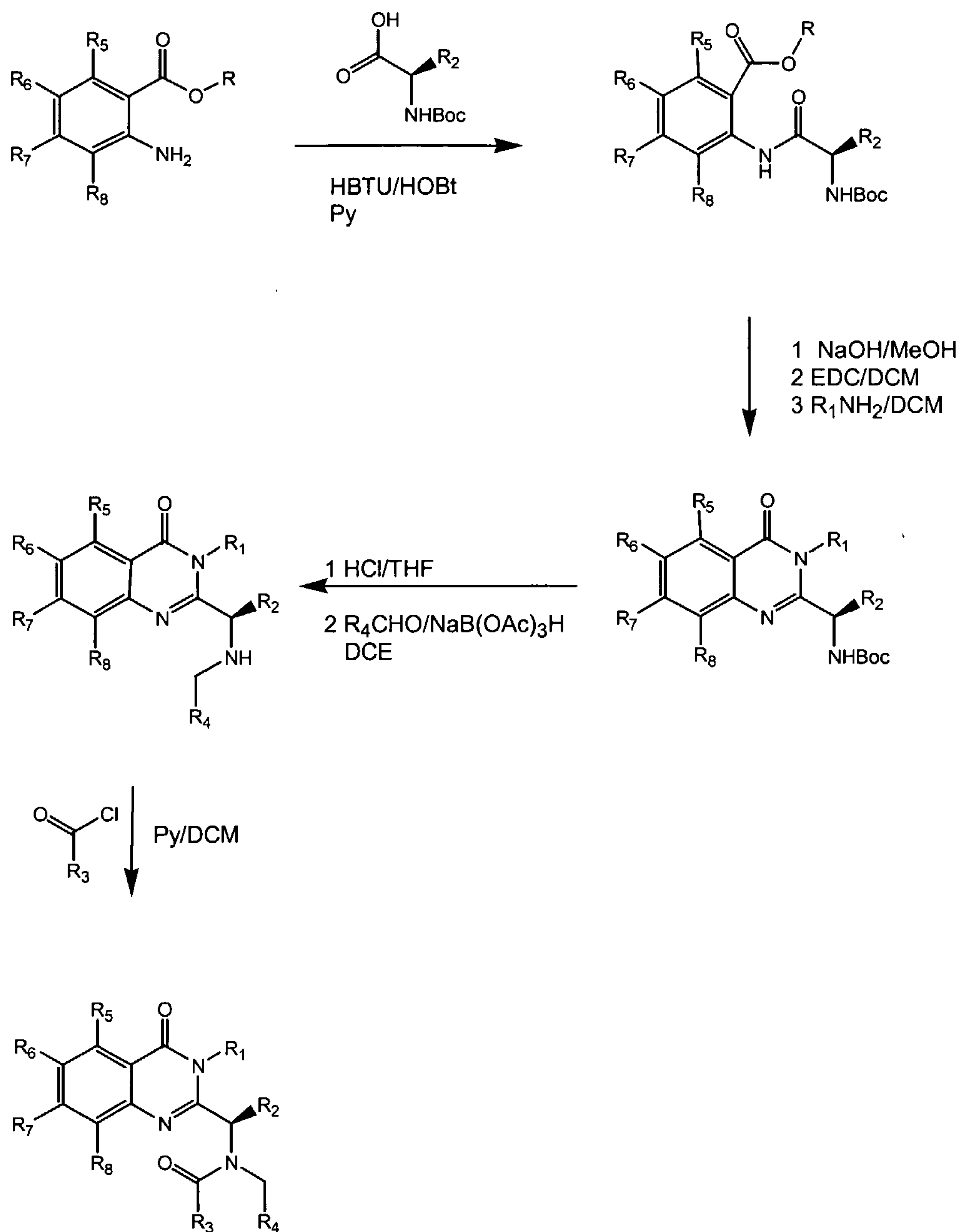
Figure 4: Asymmetric Synthesis
