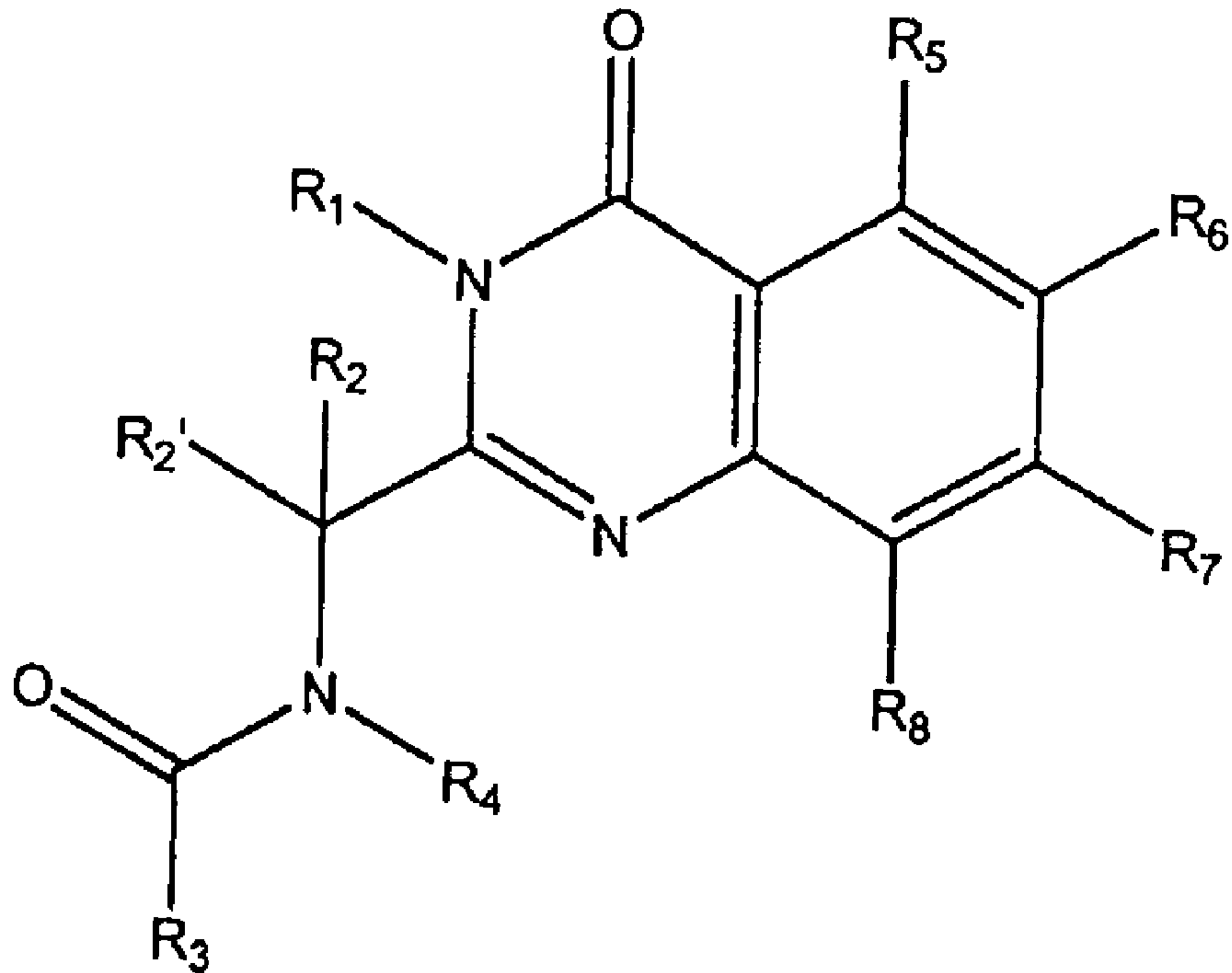
Formula 1a
