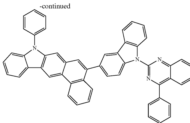
45
