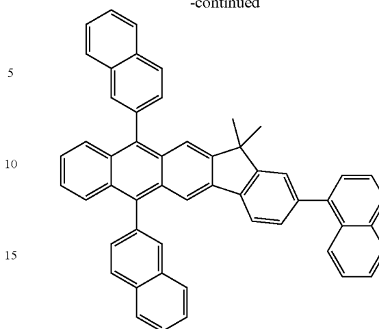
Formula 401
