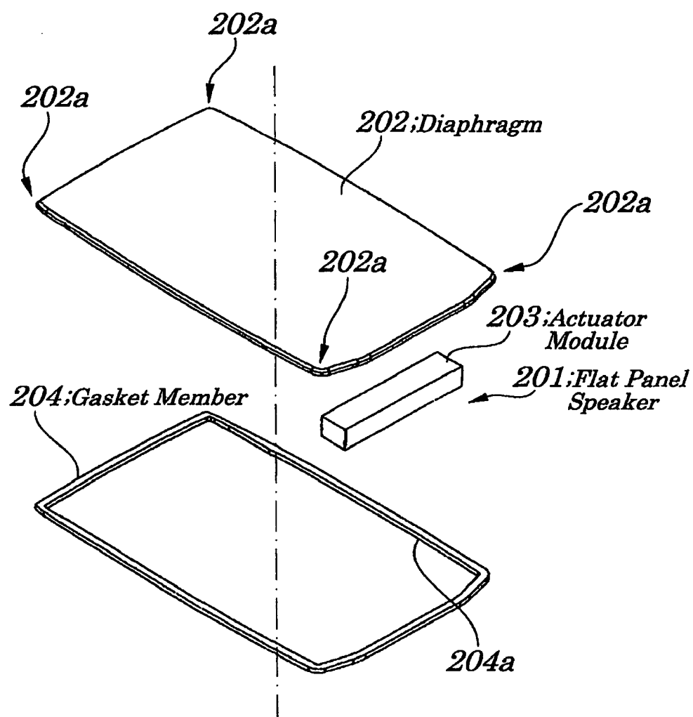
FIG. 23(PRIOR ART)
