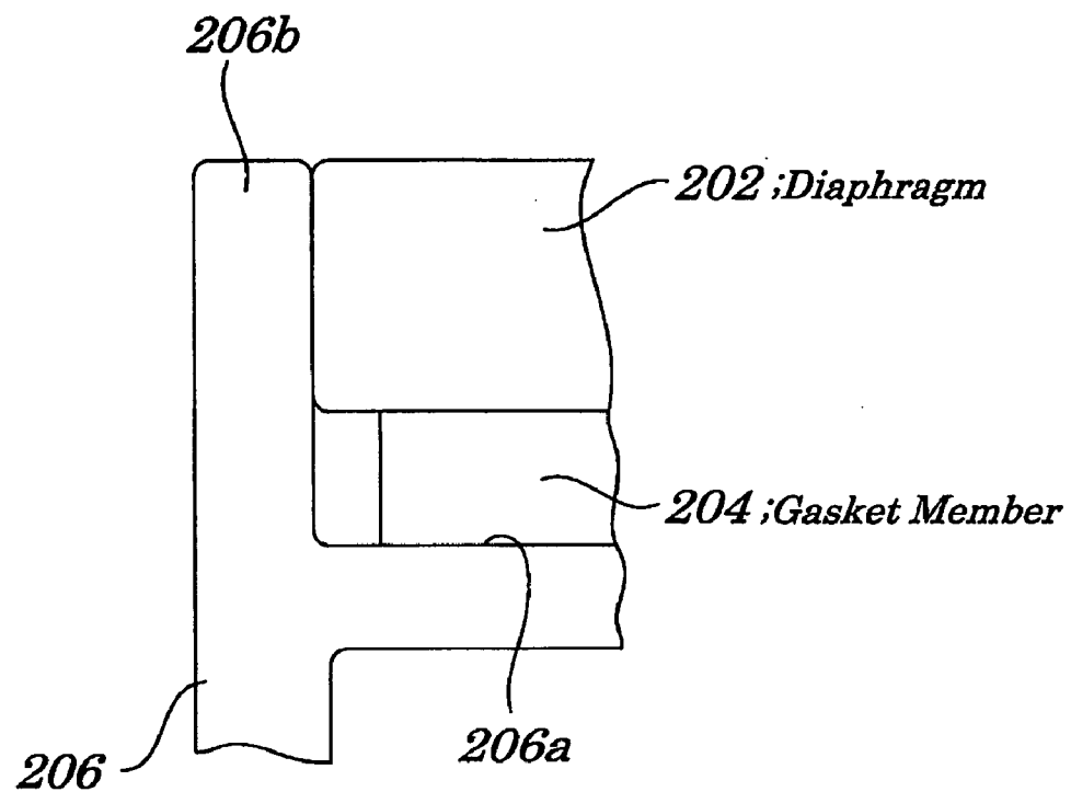
FIG.25(PRIOR ART)
