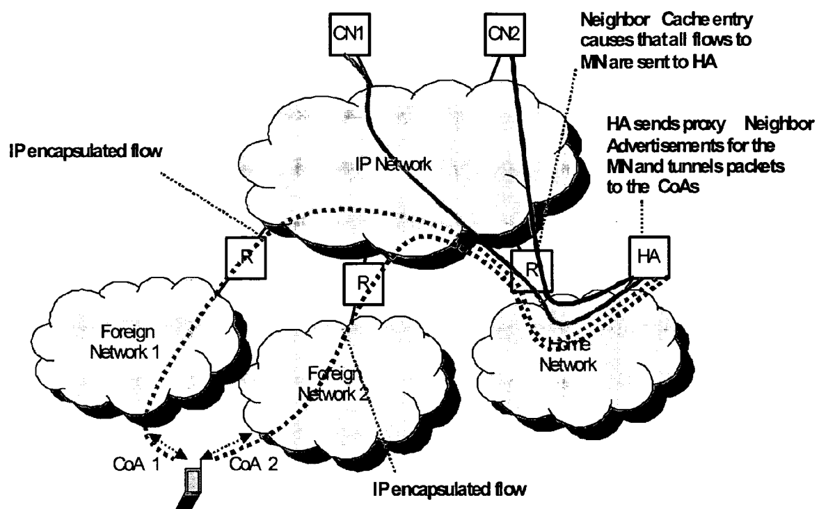
Figure 1: Use of multiple links in Foreign Networks
