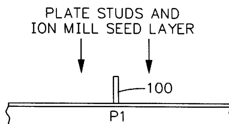
FIG. 15D (PRIOR ART)
