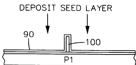
FIG. 15A (PRIOR ART)
