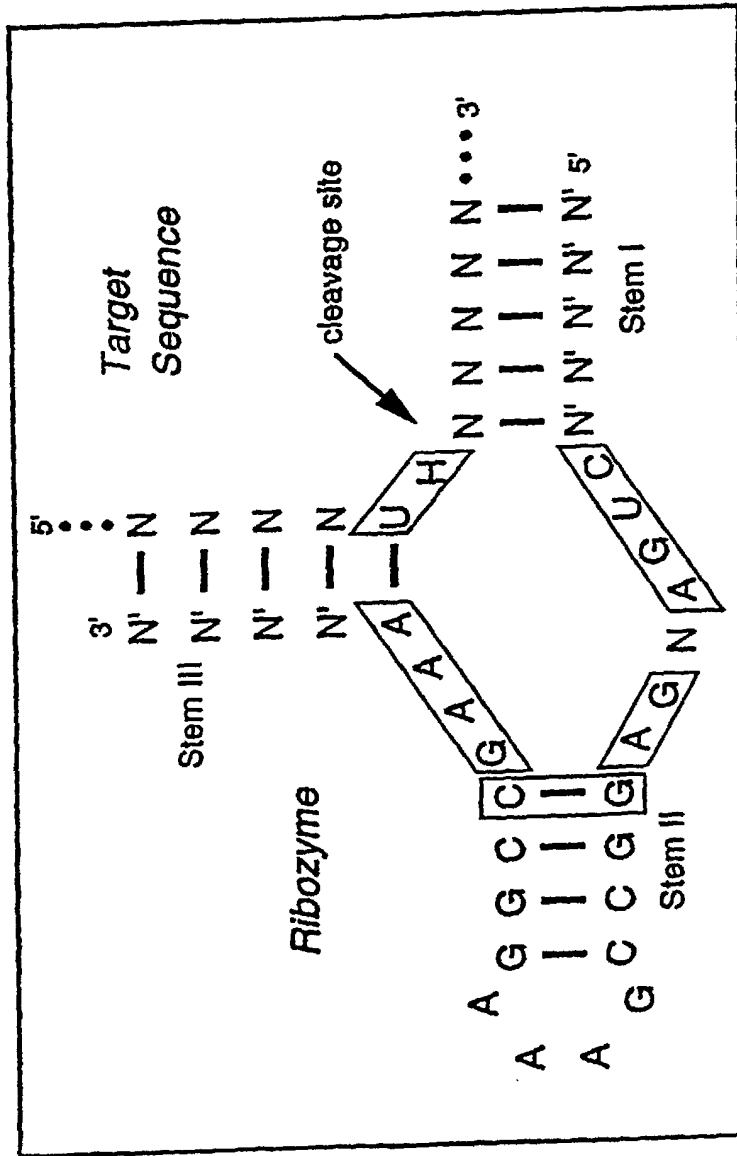
Figure 1: Hammerhead Ribozyme
