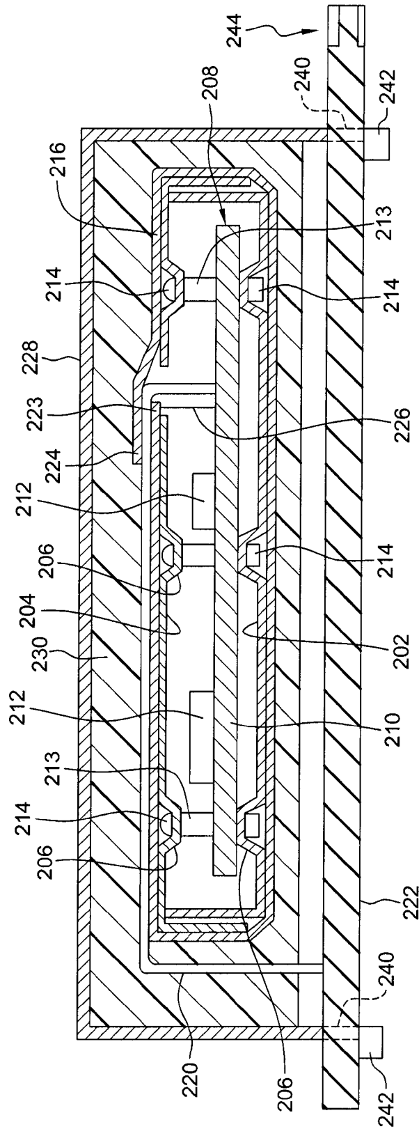
FIG. 2 (PRIOR ART)
