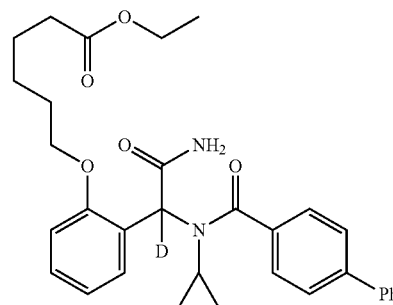
Formula 28
