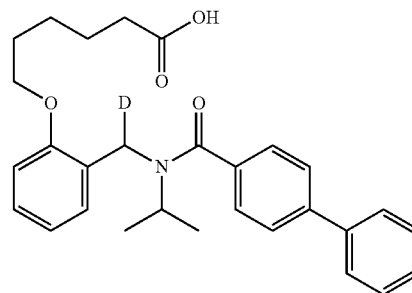
Formula 23
