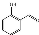
2-Salicylaldehyde
