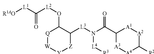
Formula 20
