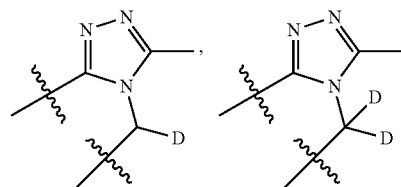
Formula 21 5
