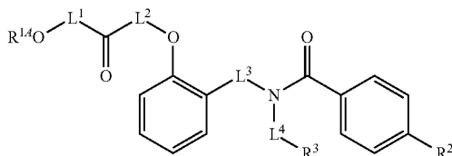
Formula 19
