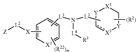
Formula 8
