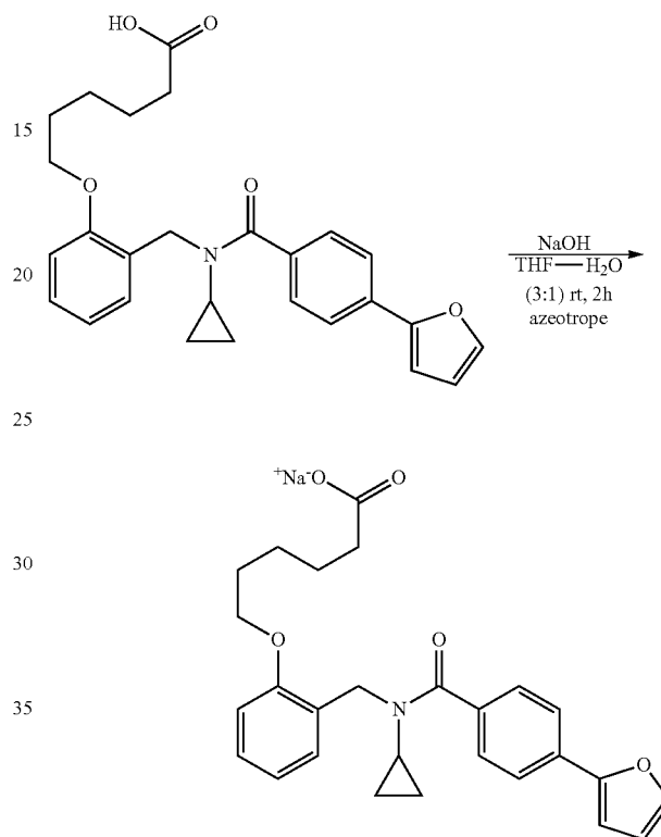
Reaction Step 6—Salt Formation
