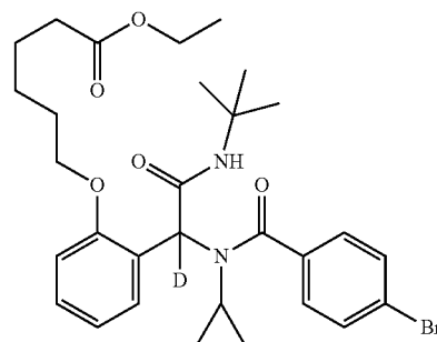
Formula 25
