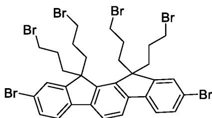
2,9-dibromo-11,11,12,12-tetrakis(3-bromopropyl)-11,12-dihydroindeno[2,1- a ]fluorene
