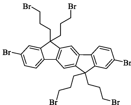
2,8-dibromo-6,6,12,12-tetrakis(3-bromopropyl)-6,12-dihydroindeno[1,2-b]fluorene
