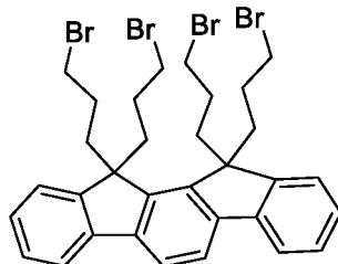
11,11,12,12-tetrakis(3-bromopropyl)-11,12-dihydroindeno[2,1- a ]fluorene
