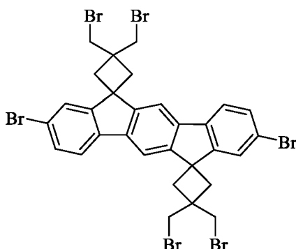
2',8'-dibromo-3,3',3"-tetrakis(bromomethyl)dispiro[cyclobutane-1,6'-indeno[1,2- b ]fluorene-12',1"-cyclobutane]
