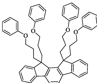
11,11,12,12-tetrakis(3-phenoxypropyl)-11,12-dihydroindeno[2,1-a]fluorene
