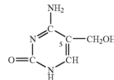
5-Hydroxymethylcytosine
