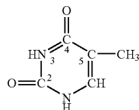
Thymine (5-methyl-2,4-dioxypyrimidine)
