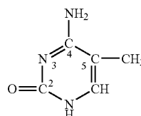
5-Methylcytosine
