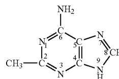
2-Methyladenine
