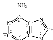
Adenosine (6-aminopurine)
