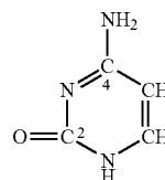
Cytosine (2-oxy-4-aminopyrimidine)
