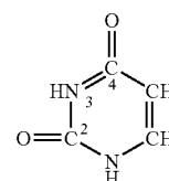
Uracil (2,4-dioxypyrimidine)
