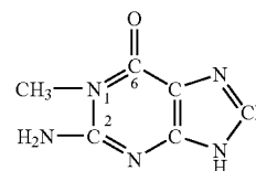
1-Methylguanine
