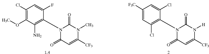
Comparative herbicidal activity of compounds 1.4 and 2
