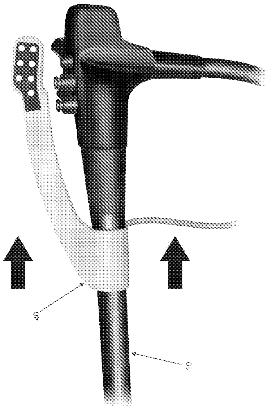
1. Slide hand piece onto scope
