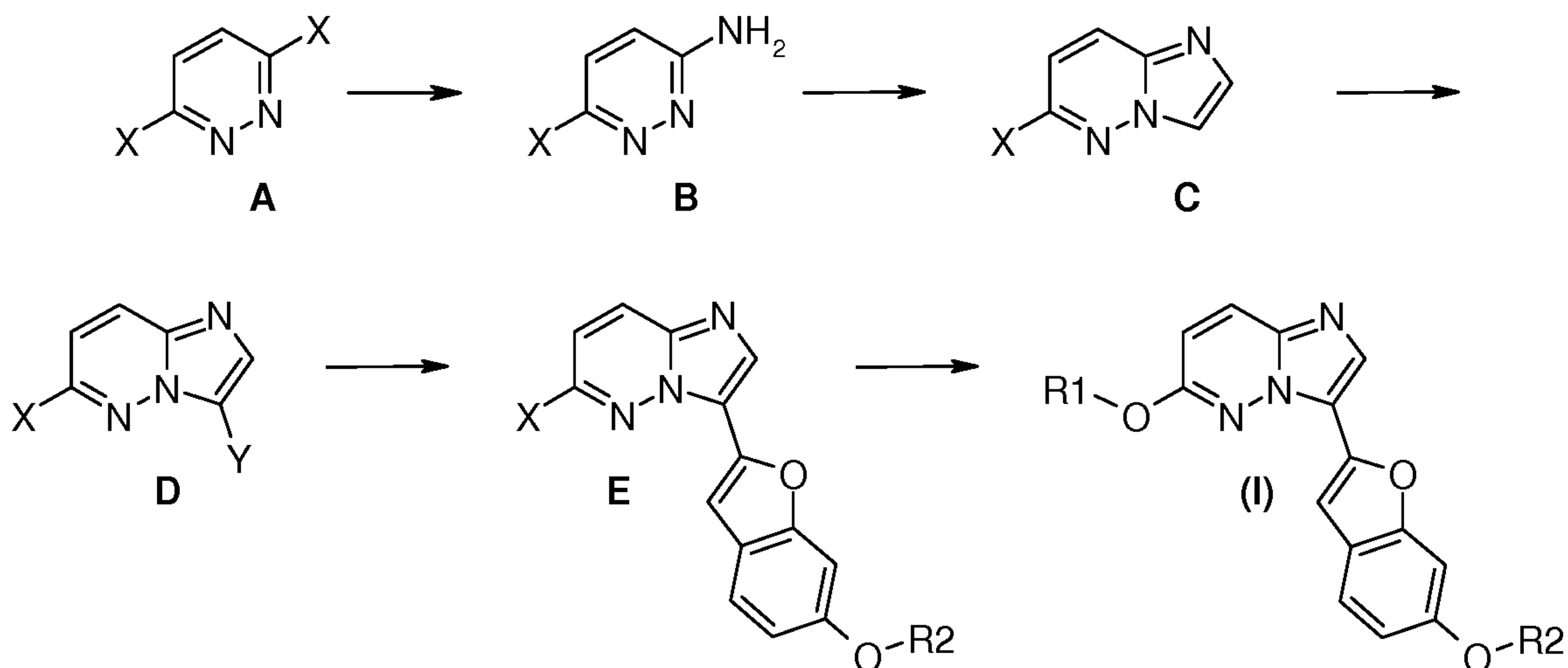
Scheme 1:
