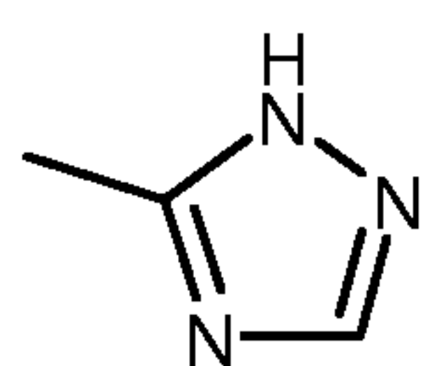
1H-tautomer
