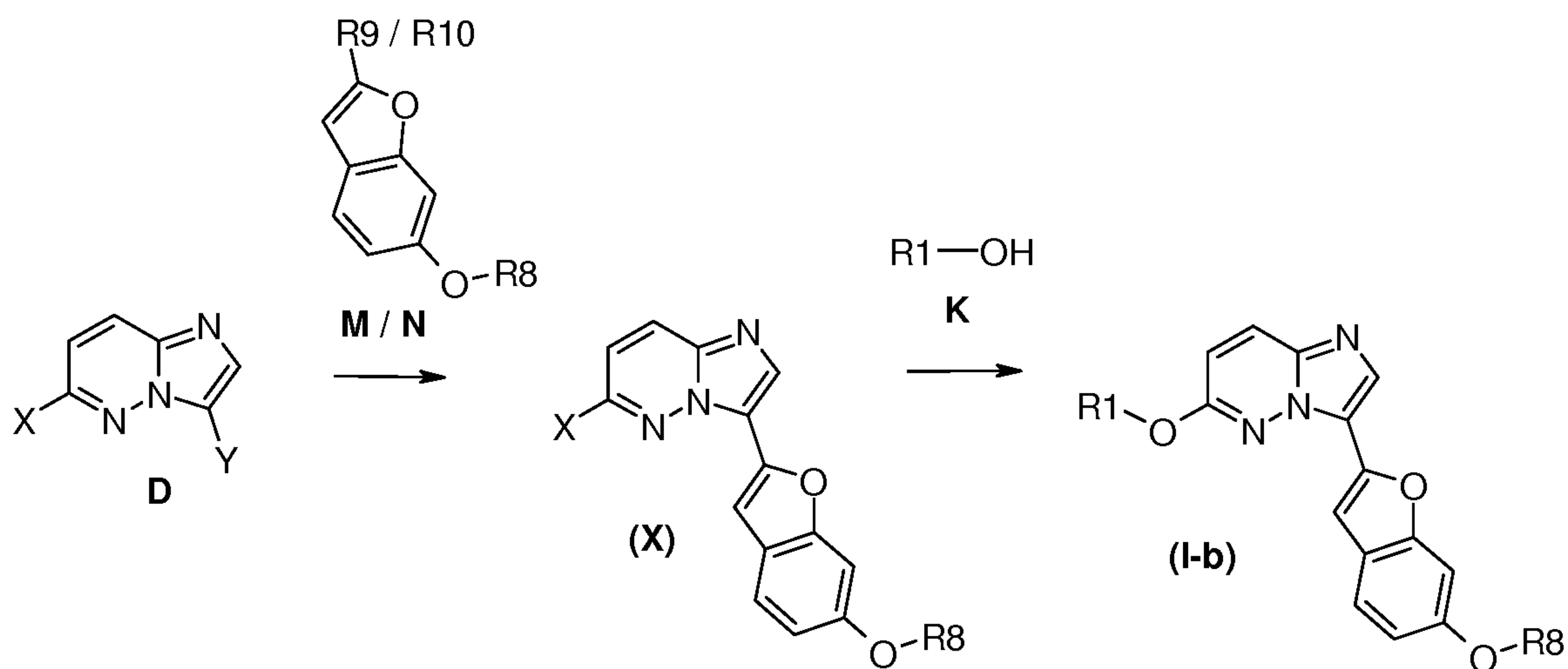
Scheme 6:
