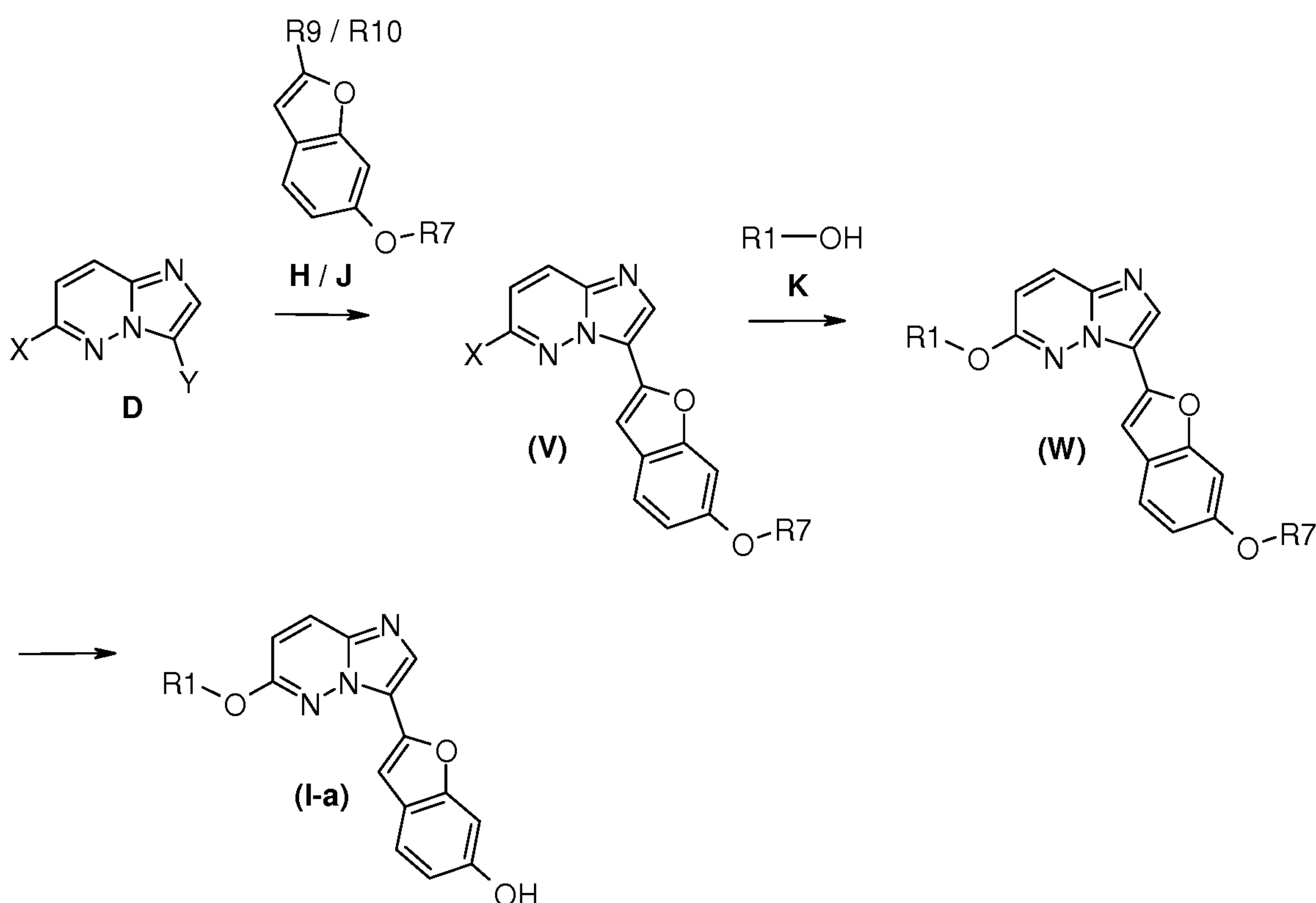
Scheme 4:
