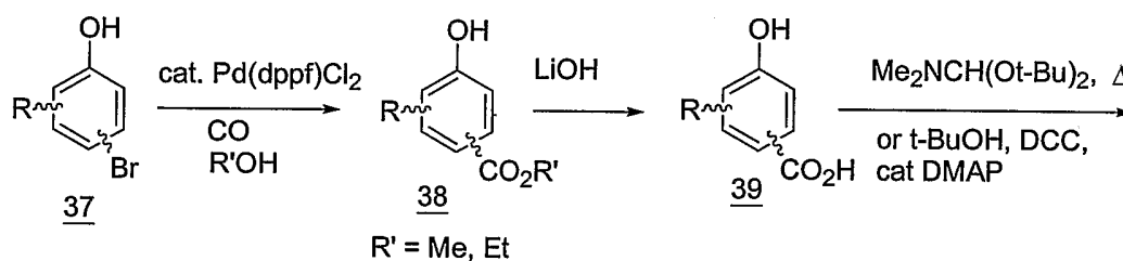
Scheme 9
