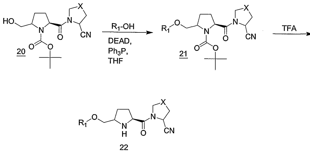
Scheme 4a
