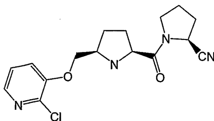
Example 45
