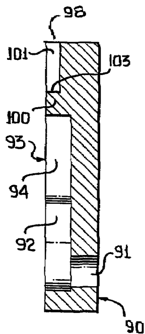
FIG. 7 Section 14-14 (PRIOR ART)
